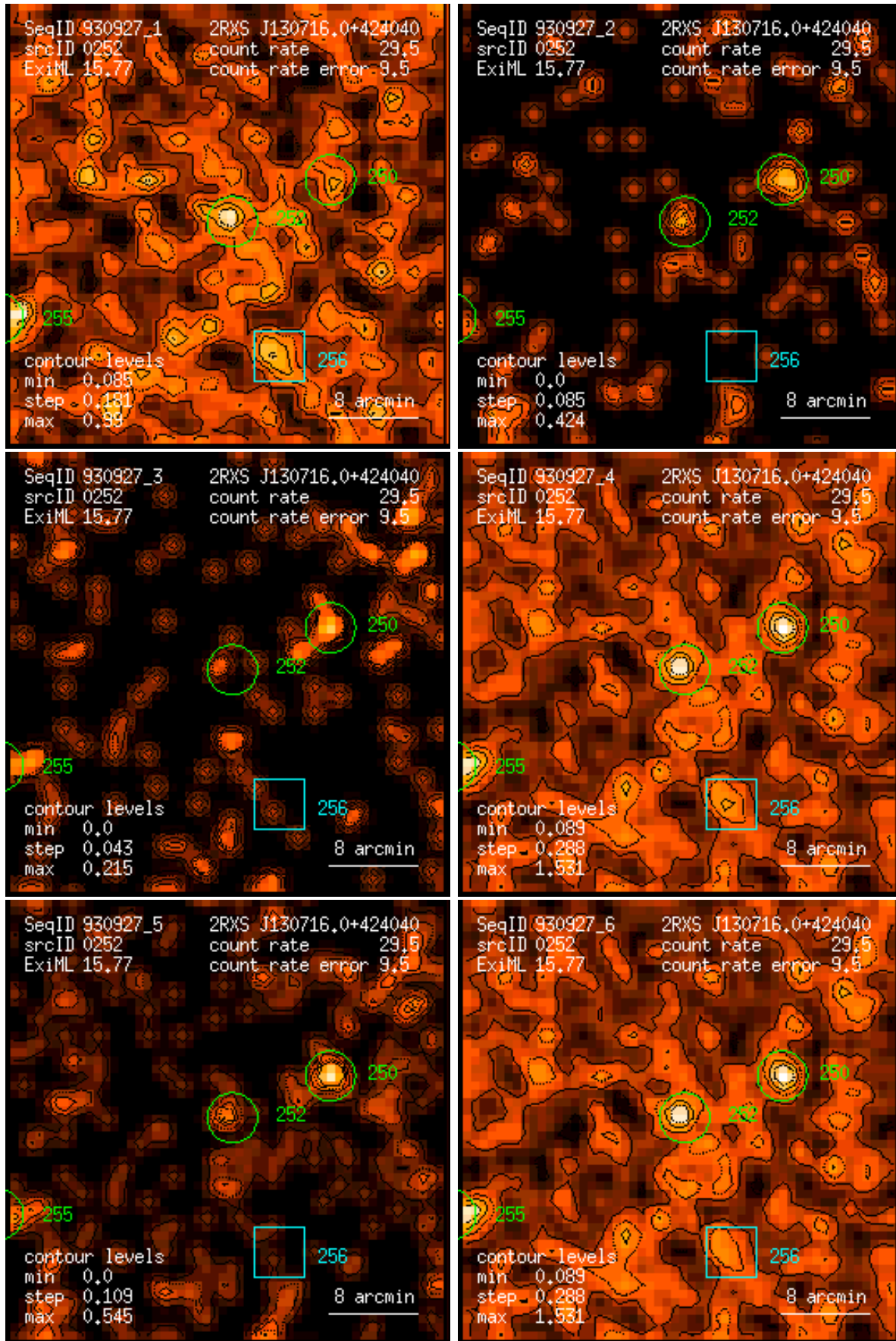
Figure 252: RASS 930927: detection 0252: band rate images, Gaussian filter: (1) PSPC channels 11 – 41, (2) 52 – 90, (3) 91 – 201, (4) 11 – 235, (5) 52 – 201, (6) 11 – 201. Broad band rates in counts/ks. Band rate contour levels in counts/ks/arcmin 2 .
