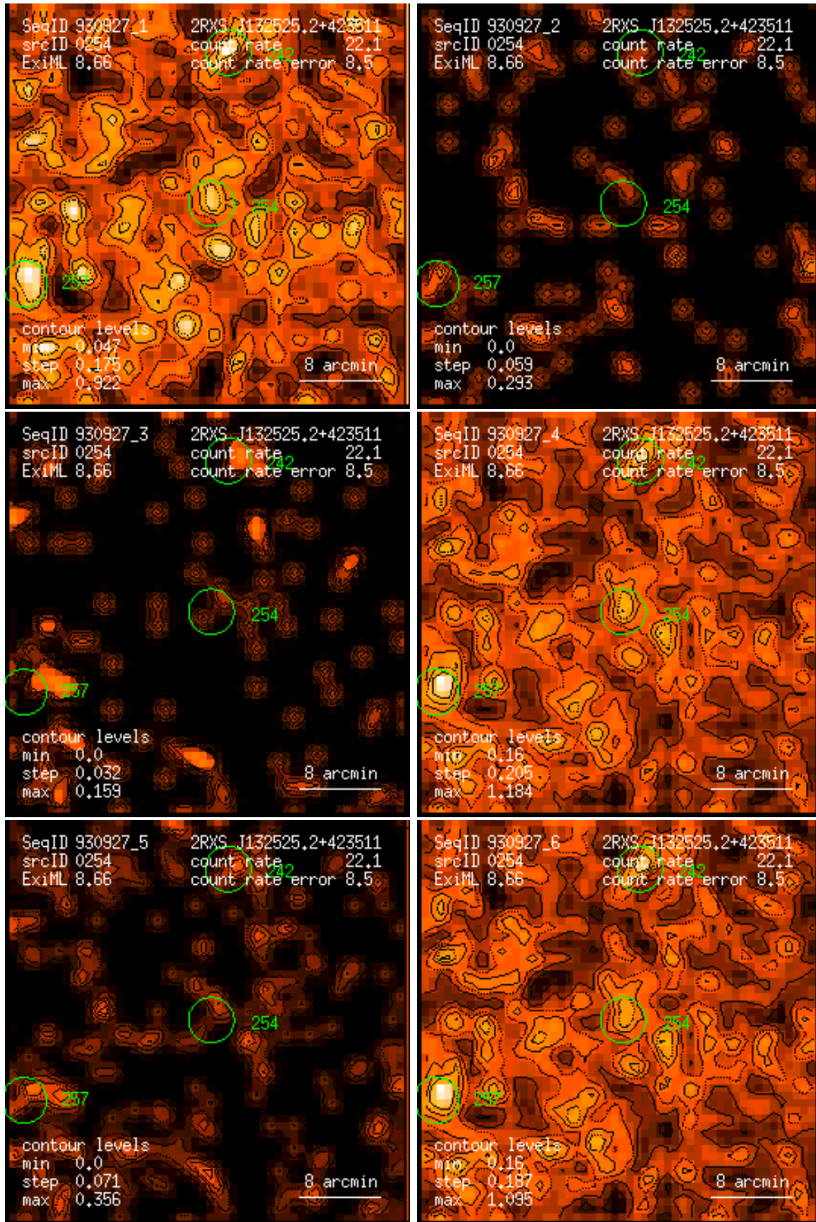
Figure 254: RASS 930927: detection 0254: band rate images, Gaussian filter: (1) PSPC channels 11 – 41, (2) 52 – 90, (3) 91 – 201, (4) 11 – 235, (5) 52 – 201, (6) 11 – 201. Broad band rates in counts/ks. Band rate contour levels in counts/ks/arcmin 2 .
