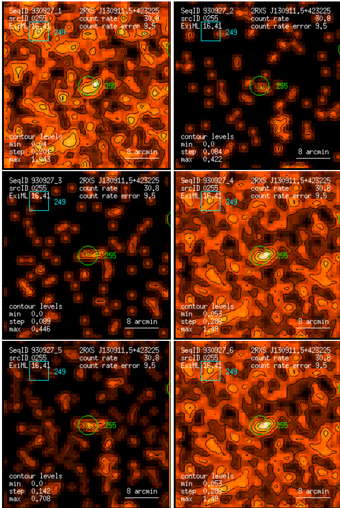
Figure 255: RASS 930927: detection 0255: band rate images, Gaussian filter: (1) PSPC channels 11 – 41, (2) 52 – 90, (3) 91 – 201, (4) 11 – 235, (5) 52 – 201, (6) 11 – 201. Broad band rates in counts/ks. Band rate contour levels in counts/ks/arcmin 2 .
