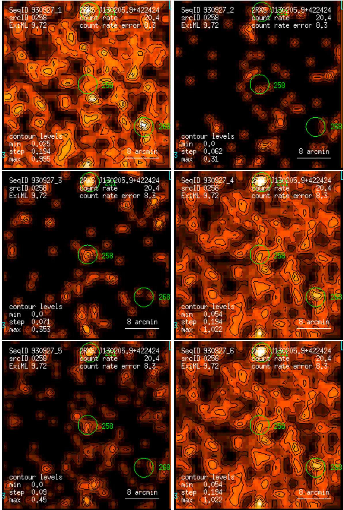
Figure 258: RASS 930927: detection 0258: band rate images, Gaussian filter: (1) PSPC channels 11 – 41, (2) 52 – 90, (3) 91 – 201, (4) 11 – 235, (5) 52 – 201, (6) 11 – 201. Broad band rates in counts/ks. Band rate contour levels in counts/ks/arcmin 2 .
