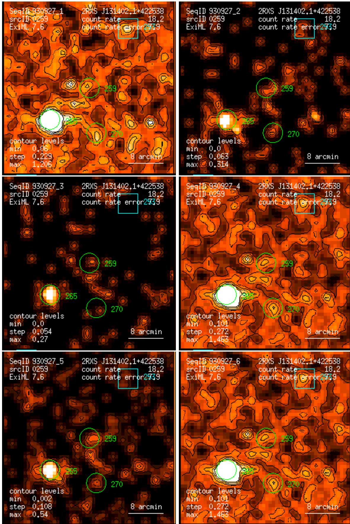
Figure 259: RASS 930927: detection 0259: band rate images, Gaussian filter: (1) PSPC channels 11 – 41, (2) 52 – 90, (3) 91 – 201, (4) 11 – 235, (5) 52 – 201, (6) 11 – 201. Broad band rates in counts/ks. Band rate contour levels in counts/ks/arcmin 2 .
