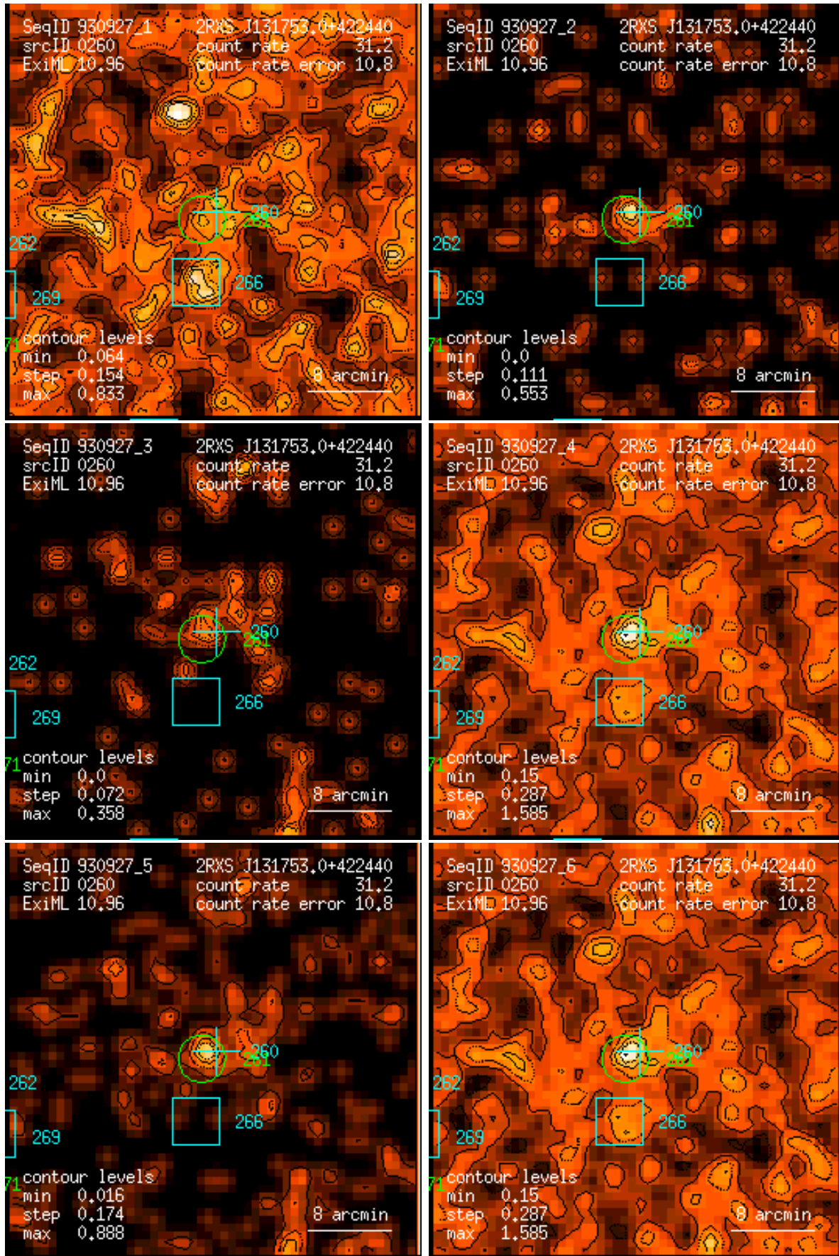
Figure 260: RASS 930927: detection 0260: band rate images, Gaussian filter: (1) PSPC channels 11 – 41, (2) 52 – 90, (3) 91 – 201, (4) 11 – 235, (5) 52 – 201, (6) 11 – 201. Broad band rates in counts/ks. Band rate contour levels in counts/ks/arcmin 2 .
