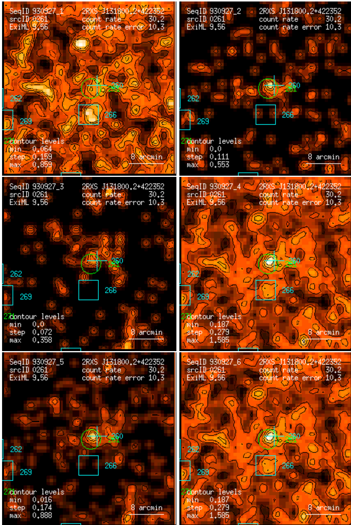
Figure 261: RASS 930927: detection 0261: band rate images, Gaussian filter: (1) PSPC channels 11 – 41, (2) 52 – 90, (3) 91 – 201, (4) 11 – 235, (5) 52 – 201, (6) 11 – 201. Broad band rates in counts/ks. Band rate contour levels in counts/ks/arcmin 2 .
