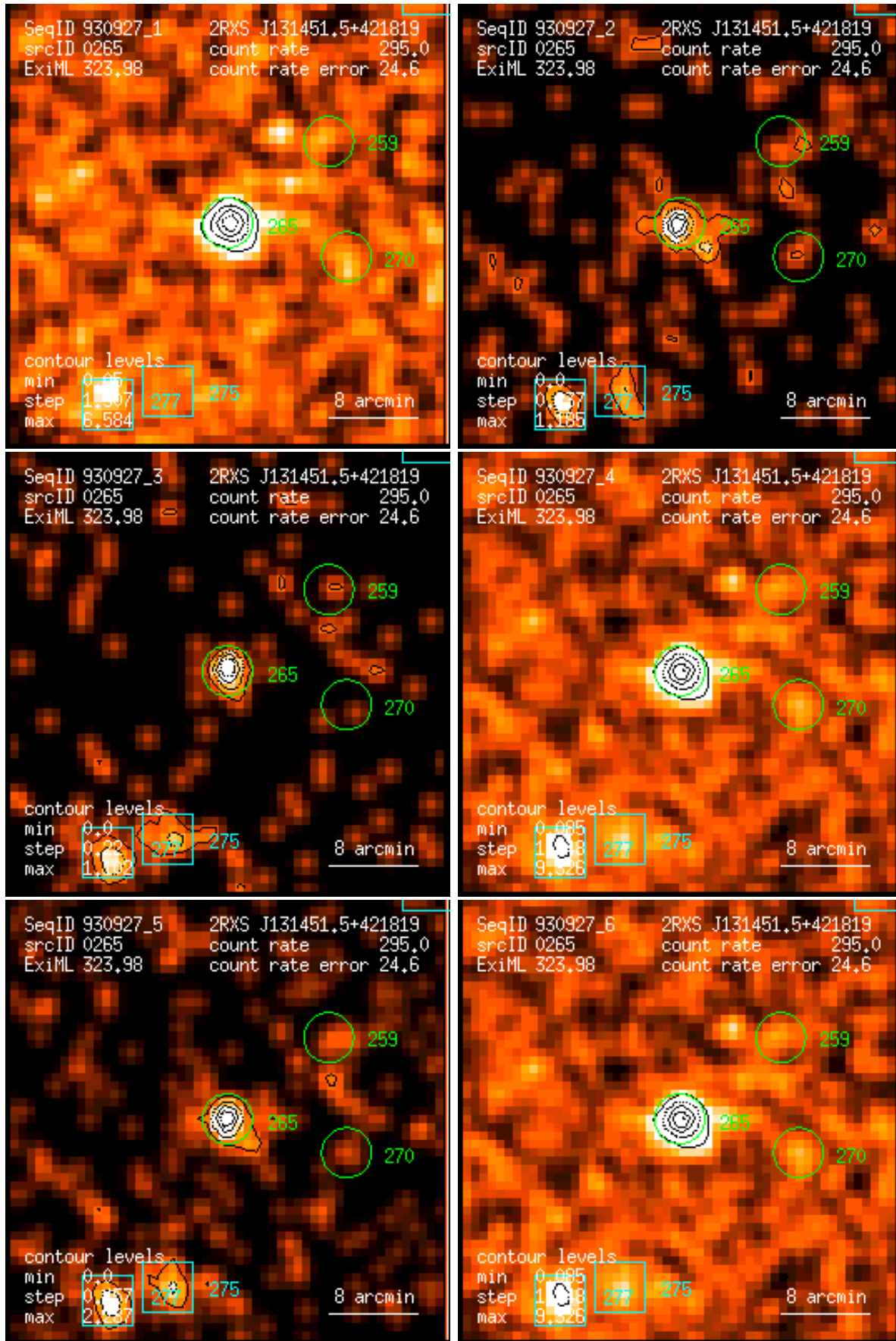
Figure 265: RASS 930927: detection 0265: band rate images, Gaussian filter: (1) PSPC channels 11 – 41, (2) 52 – 90, (3) 91 – 201, (4) 11 – 235, (5) 52 – 201, (6) 11 – 201. Broad band rates in counts/ks. Band rate contour levels in counts/ks/arcmin 2 .
