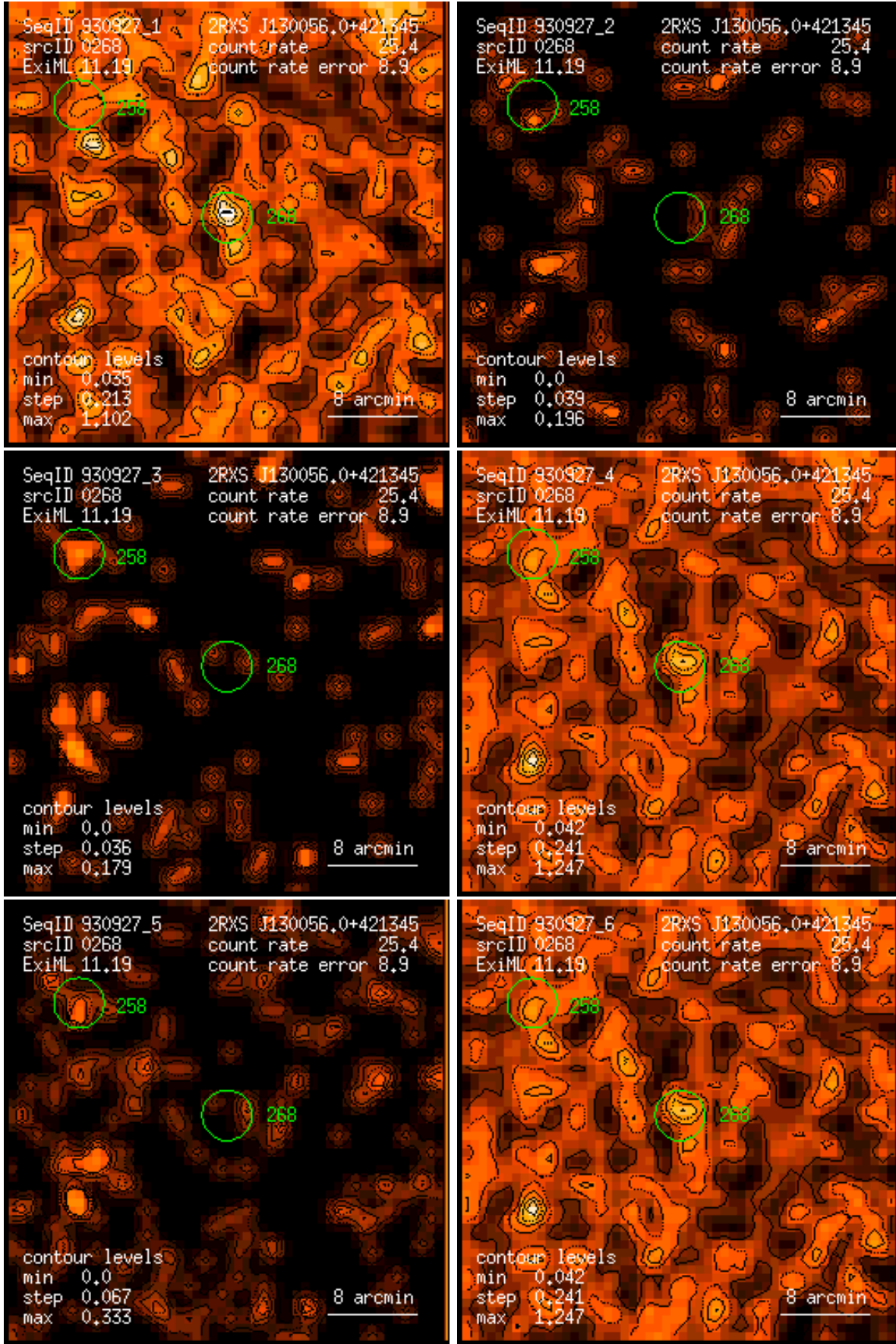
Figure 268: RASS 930927: detection 0268: band rate images, Gaussian filter: (1) PSPC channels 11 – 41, (2) 52 – 90, (3) 91 – 201, (4) 11 – 235, (5) 52 – 201, (6) 11 – 201. Broad band rates in counts/ks. Band rate contour levels in counts/ks/arcmin 2 .
