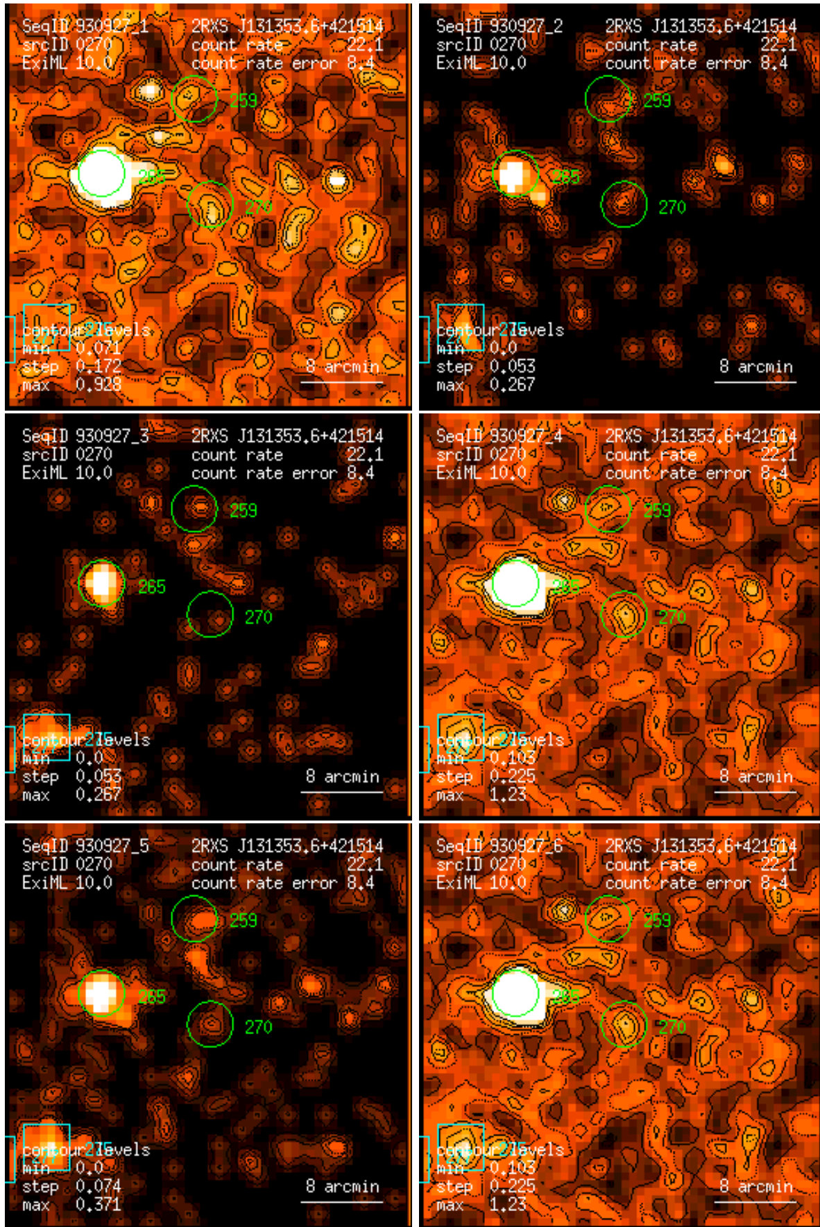
Figure 270: RASS 930927: detection 0270: band rate images, Gaussian filter: (1) PSPC channels 11 – 41, (2) 52 – 90, (3) 91 – 201, (4) 11 – 235, (5) 52 – 201, (6) 11 – 201. Broad band rates in counts/ks. Band rate contour levels in counts/ks/arcmin 2 .
