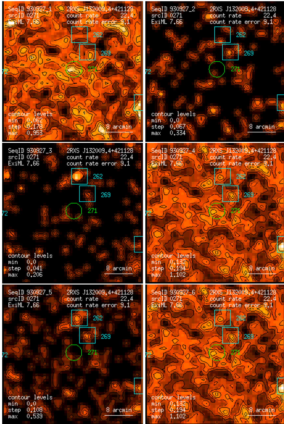
Figure 271: RASS 930927: detection 0271: band rate images, Gaussian filter: (1) PSPC channels 11 – 41, (2) 52 – 90, (3) 91 – 201, (4) 11 – 235, (5) 52 – 201, (6) 11 – 201. Broad band rates in counts/ks. Band rate contour levels in counts/ks/arcmin 2 .
