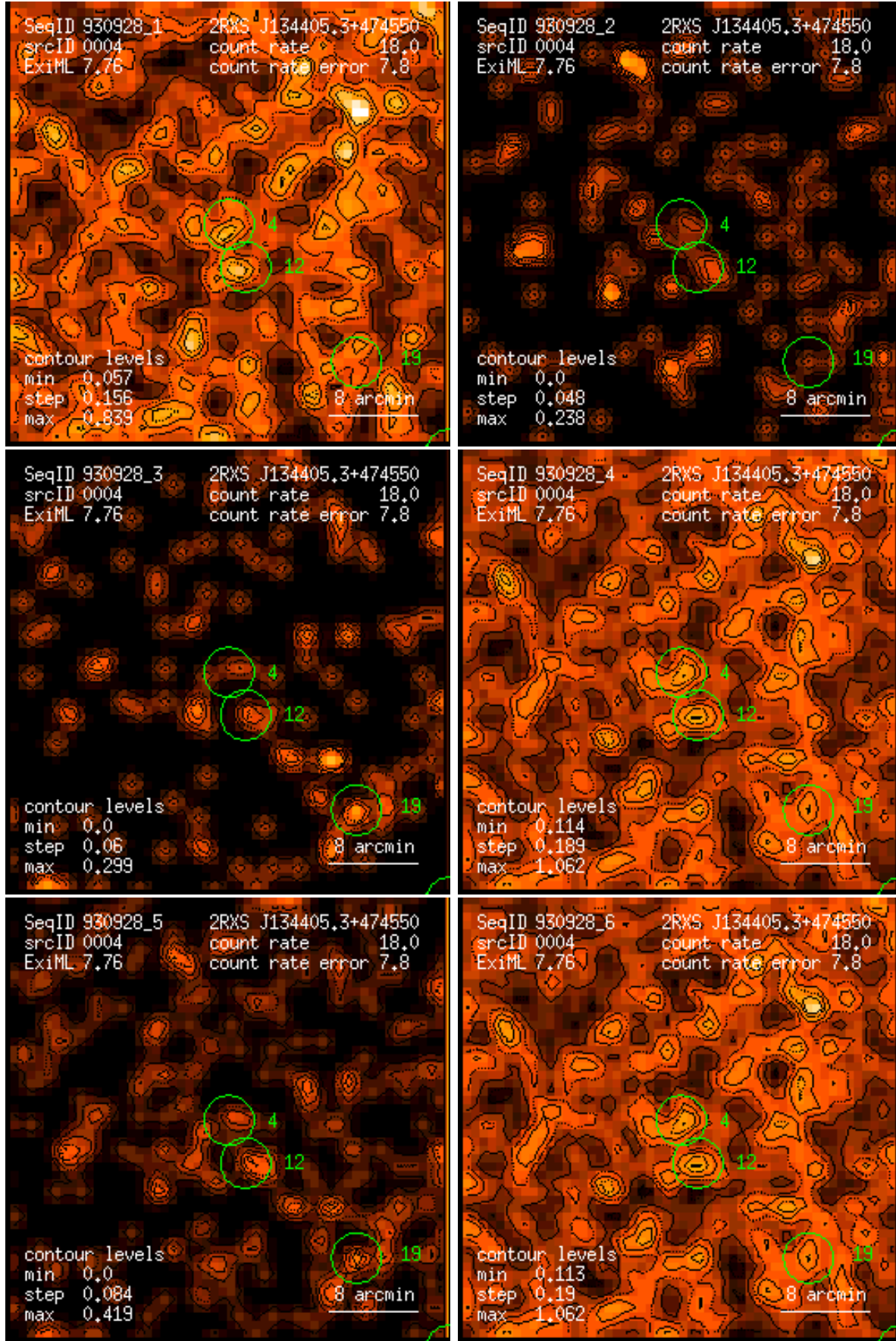
Figure 4: RASS 930928: detection 0004: band rate images, Gaussian filter: (1) PSPC channels 11 – 41, (2) 52 – 90, (3) 91 – 201, (4) 11 – 235, (5) 52 – 201, (6) 11 – 201. Broad band rates in counts/ks. Band rate contour levels in counts/ks/arcmin 2 .
