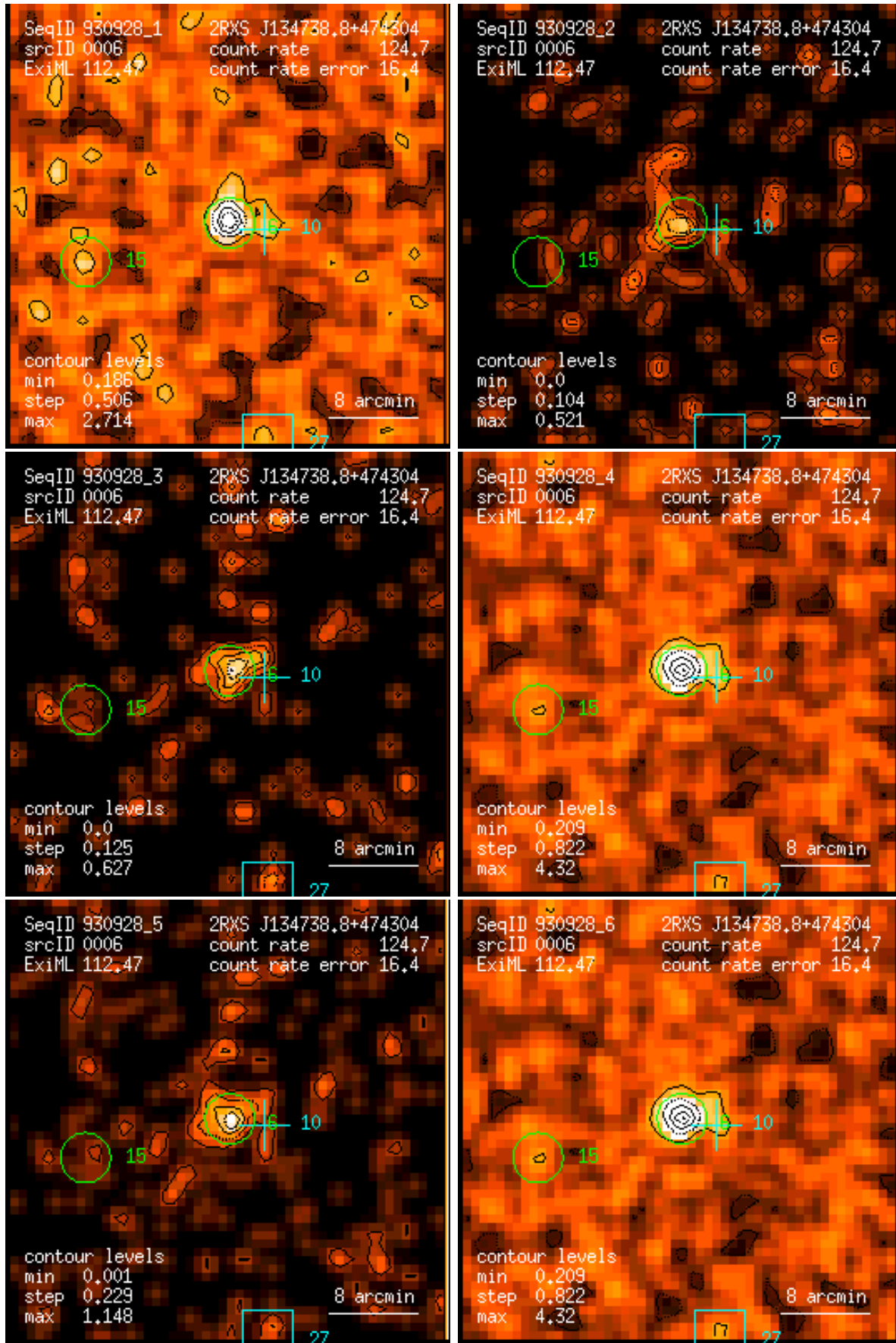
Figure 6: RASS 930928: detection 0006: band rate images, Gaussian filter: (1) PSPC channels 11 – 41, (2) 52 – 90, (3) 91 – 201, (4) 11 – 235, (5) 52 – 201, (6) 11 – 201. Broad band rates in counts/ks. Band rate contour levels in counts/ks/arcmin 2 .
