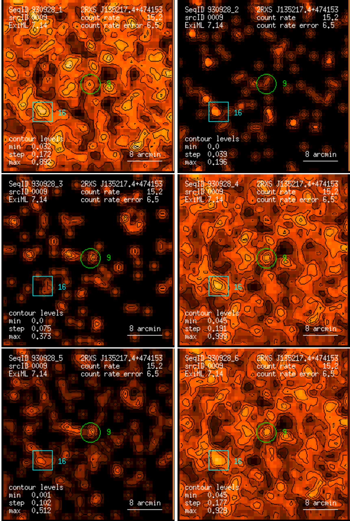
Figure 9: RASS 930928: detection 0009: band rate images, Gaussian filter: (1) PSPC channels 11 – 41, (2) 52 – 90, (3) 91 – 201, (4) 11 – 235, (5) 52 – 201, (6) 11 – 201. Broad band rates in counts/ks. Band rate contour levels in counts/ks/arcmin 2 .
