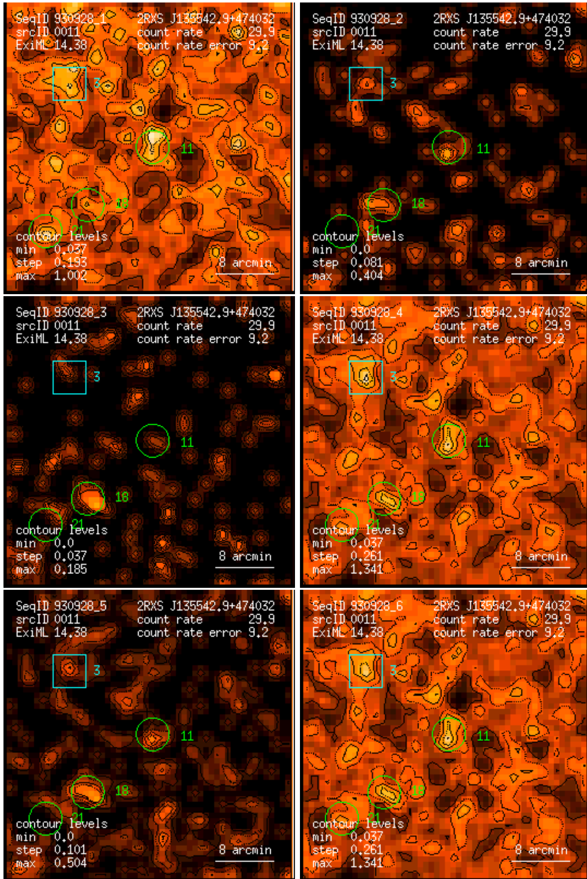
Figure 11: RASS 930928: detection 0011: band rate images, Gaussian filter: (1) PSPC channels 11 – 41, (2) 52 – 90, (3) 91 – 201, (4) 11 – 235, (5) 52 – 201, (6) 11 – 201. Broad band rates in counts/ks. Band rate contour levels in counts/ks/arcmin 2 .
