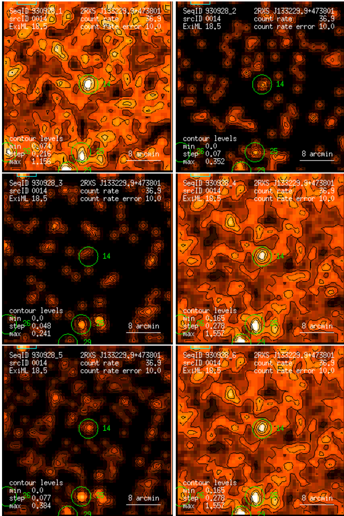
Figure 14: RASS 930928: detection 0014: band rate images, Gaussian filter: (1) PSPC channels 11 – 41, (2) 52 – 90, (3) 91 – 201, (4) 11 – 235, (5) 52 – 201, (6) 11 – 201. Broad band rates in counts/ks. Band rate contour levels in counts/ks/arcmin 2 .
