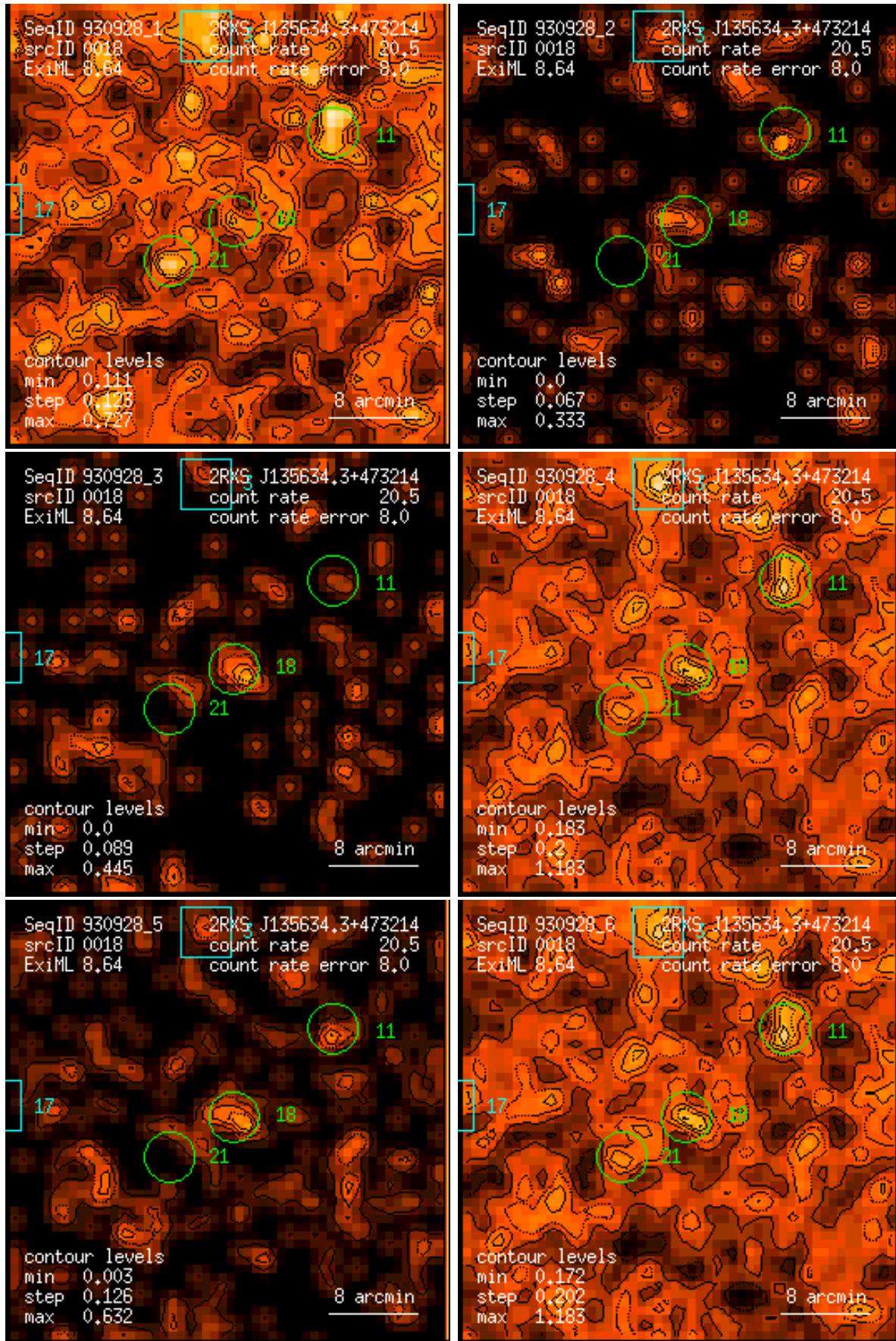
Figure 18: RASS 930928: detection 0018: band rate images, Gaussian filter: (1) PSPC channels 11 – 41, (2) 52 – 90, (3) 91 – 201, (4) 11 – 235, (5) 52 – 201, (6) 11 – 201. Broad band rates in counts/ks. Band rate contour levels in counts/ks/arcmin 2 .
