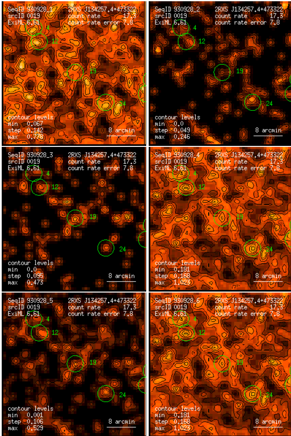
Figure 19: RASS 930928: detection 0019: band rate images, Gaussian filter: (1) PSPC channels 11 – 41, (2) 52 – 90, (3) 91 – 201, (4) 11 – 235, (5) 52 – 201, (6) 11 – 201. Broad band rates in counts/ks. Band rate contour levels in counts/ks/arcmin 2 .
