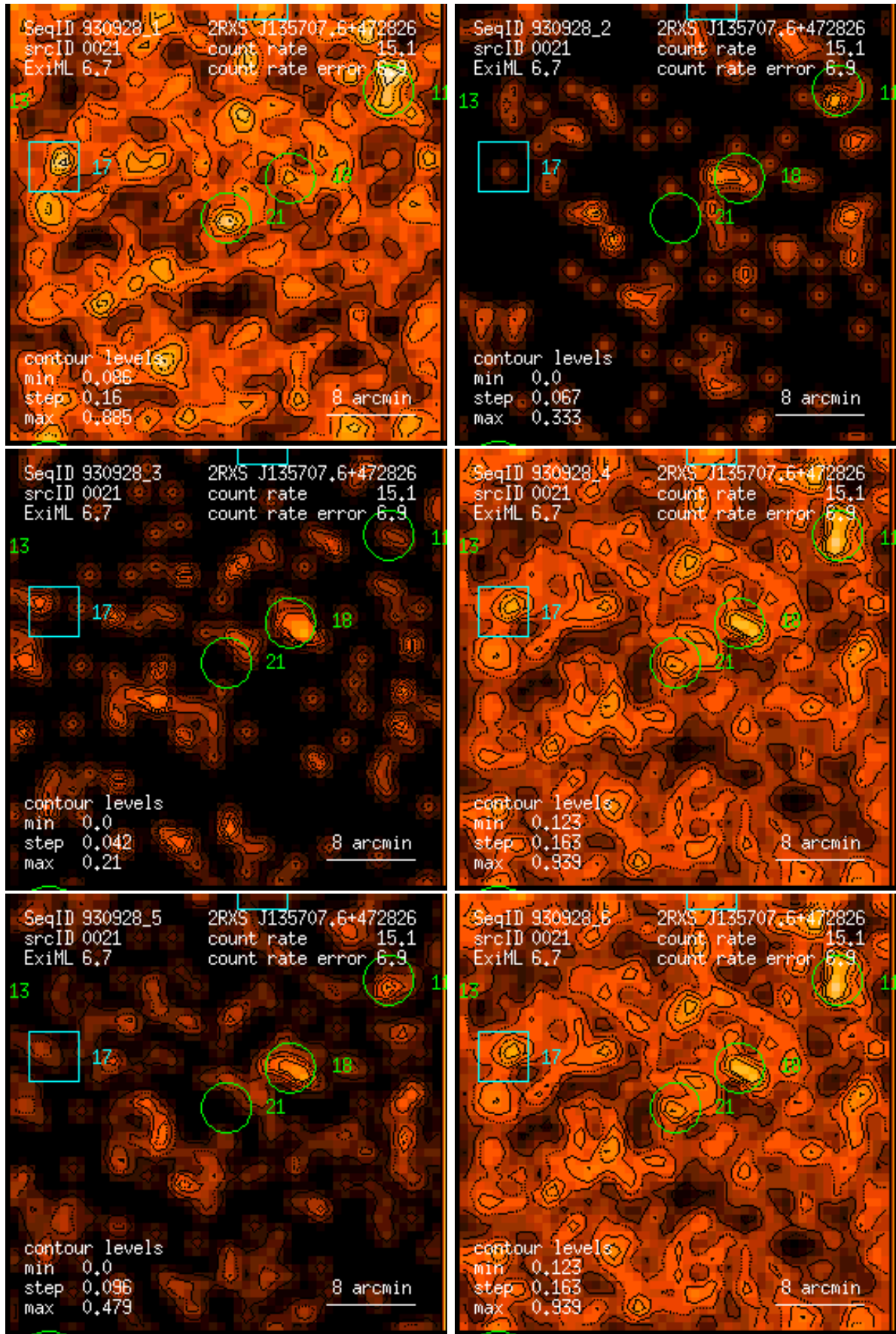
Figure 21: RASS 930928: detection 0021: band rate images, Gaussian filter: (1) PSPC channels 11 – 41, (2) 52 – 90, (3) 91 – 201, (4) 11 – 235, (5) 52 – 201, (6) 11 – 201. Broad band rates in counts/ks. Band rate contour levels in counts/ks/arcmin 2 .
