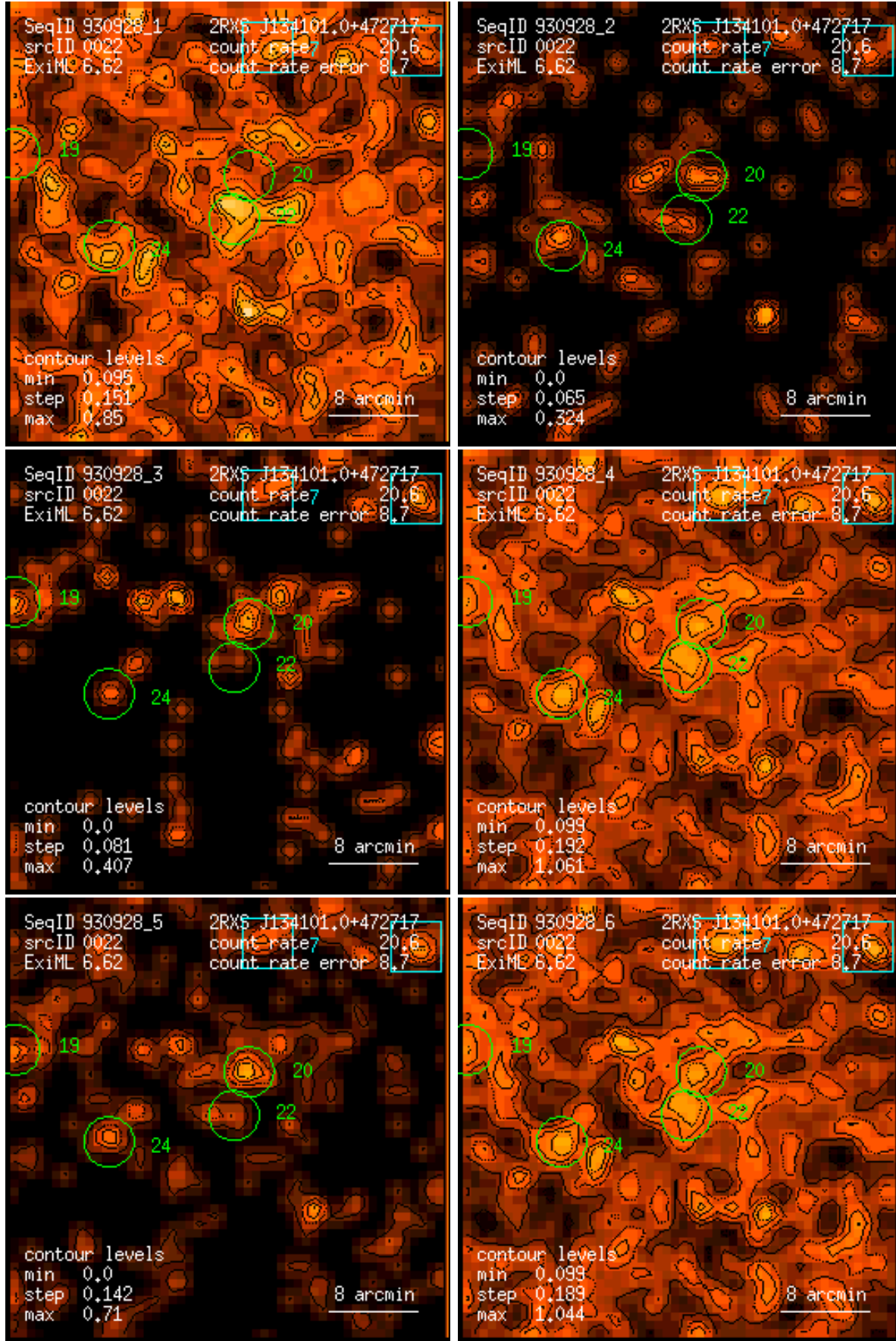
Figure 22: RASS 930928: detection 0022: band rate images, Gaussian filter: (1) PSPC channels 11 – 41, (2) 52 – 90, (3) 91 – 201, (4) 11 – 235, (5) 52 – 201, (6) 11 – 201. Broad band rates in counts/ks. Band rate contour levels in counts/ks/arcmin 2 .
