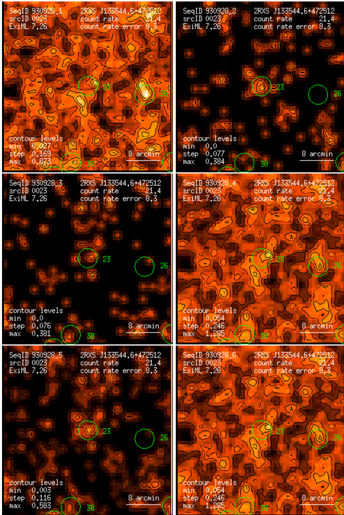
Figure 23: RASS 930928: detection 0023: band rate images, Gaussian filter: (1) PSPC channels 11 – 41, (2) 52 – 90, (3) 91 – 201, (4) 11 – 235, (5) 52 – 201, (6) 11 – 201. Broad band rates in counts/ks. Band rate contour levels in counts/ks/arcmin 2 .
