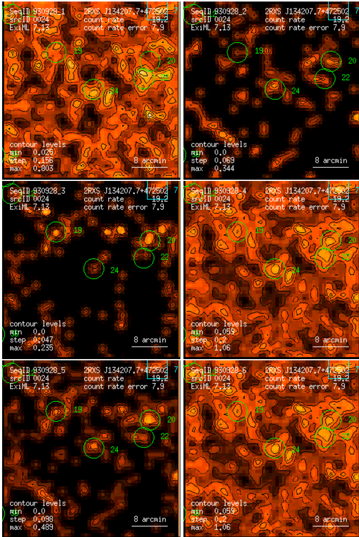
Figure 24: RASS 930928: detection 0024: band rate images, Gaussian filter: (1) PSPC channels 11 – 41, (2) 52 – 90, (3) 91 – 201, (4) 11 – 235, (5) 52 – 201, (6) 11 – 201. Broad band rates in counts/ks. Band rate contour levels in counts/ks/arcmin 2 .
