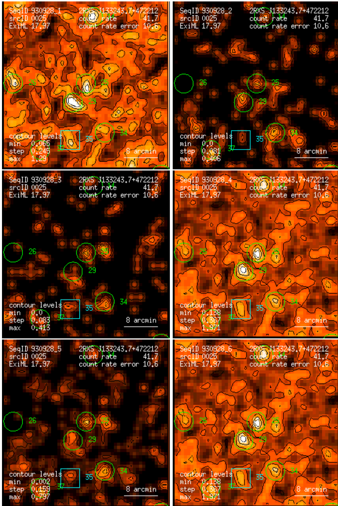
Figure 25: RASS 930928: detection 0025: band rate images, Gaussian filter: (1) PSPC channels 11 – 41, (2) 52 – 90, (3) 91 – 201, (4) 11 – 235, (5) 52 – 201, (6) 11 – 201. Broad band rates in counts/ks. Band rate contour levels in counts/ks/arcmin 2 .
