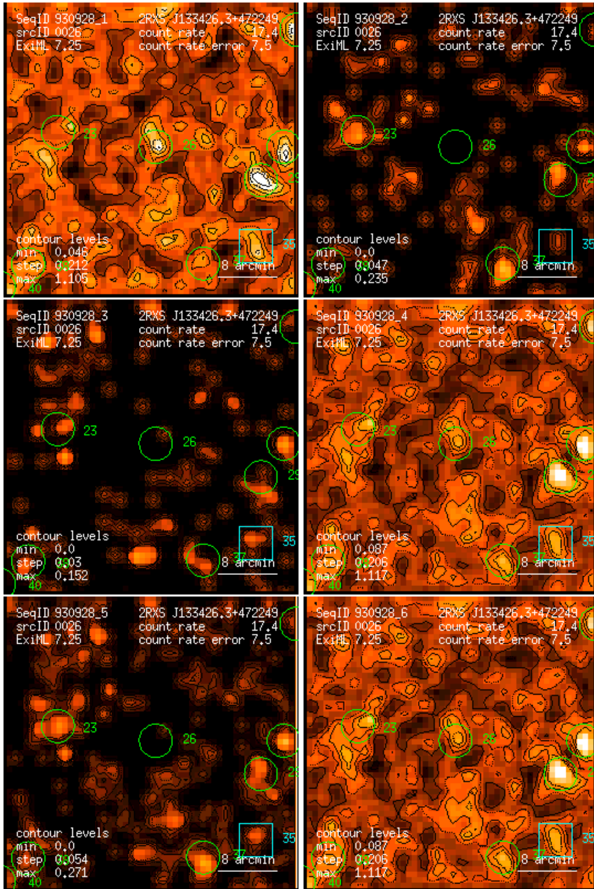
Figure 26: RASS 930928: detection 0026: band rate images, Gaussian filter: (1) PSPC channels 11 – 41, (2) 52 – 90, (3) 91 – 201, (4) 11 – 235, (5) 52 – 201, (6) 11 – 201. Broad band rates in counts/ks. Band rate contour levels in counts/ks/arcmin 2 .
