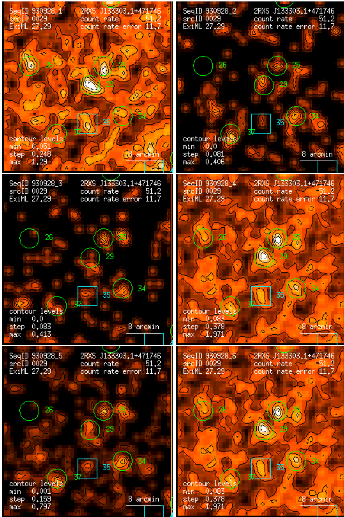
Figure 29: RASS 930928: detection 0029: band rate images, Gaussian filter: (1) PSPC channels 11 – 41, (2) 52 – 90, (3) 91 – 201, (4) 11 – 235, (5) 52 – 201, (6) 11 – 201. Broad band rates in counts/ks. Band rate contour levels in counts/ks/arcmin 2 .
