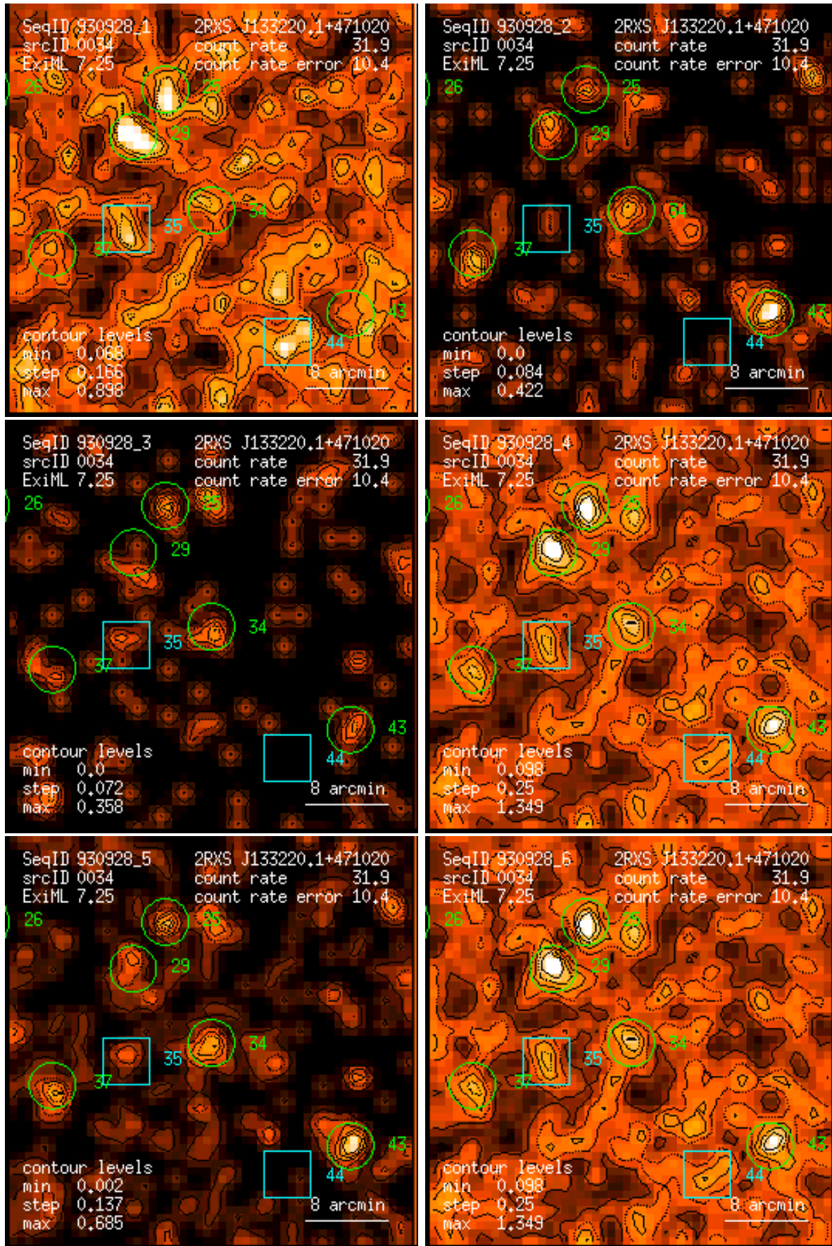
Figure 34: RASS 930928: detection 0034: band rate images, Gaussian filter: (1) PSPC channels 11 – 41, (2) 52 – 90, (3) 91 – 201, (4) 11 – 235, (5) 52 – 201, (6) 11 – 201. Broad band rates in counts/ks. Band rate contour levels in counts/ks/arcmin 2 .
