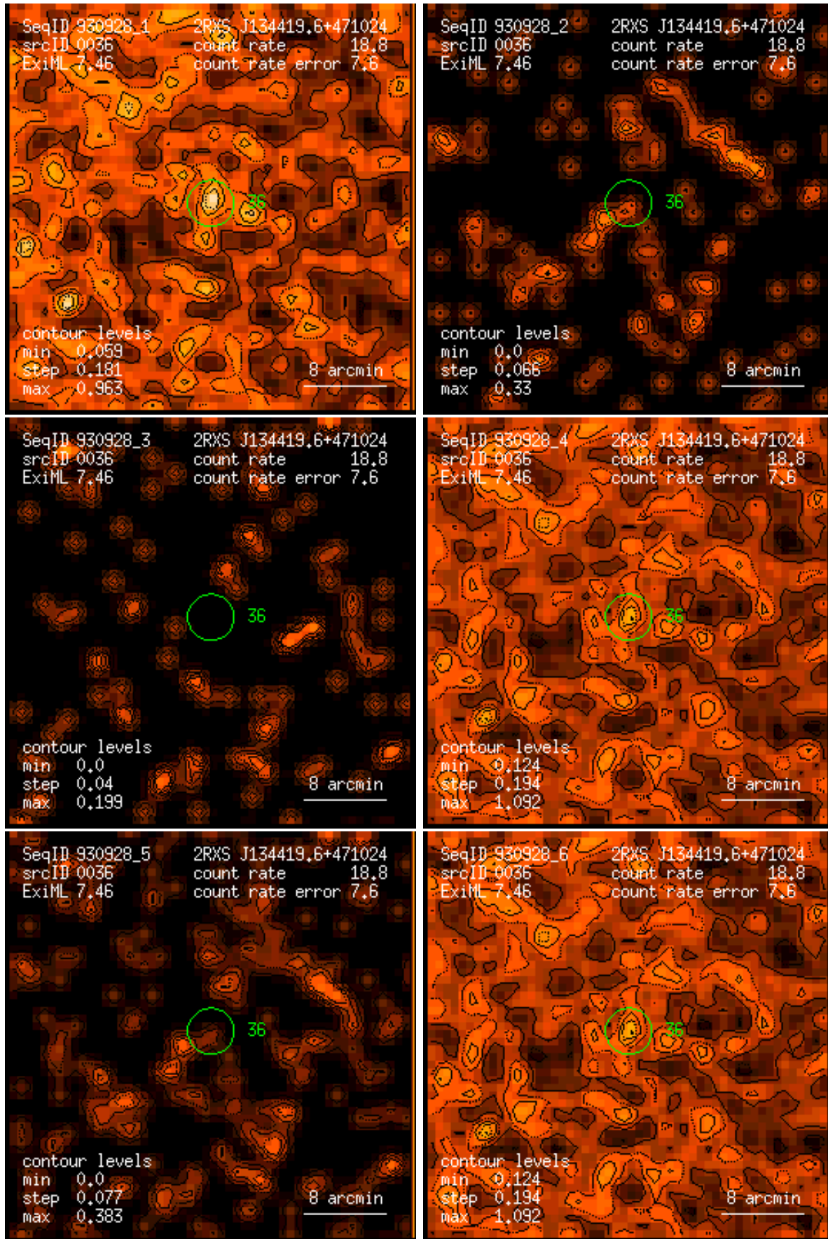
Figure 36: RASS 930928: detection 0036: band rate images, Gaussian filter: (1) PSPC channels 11 – 41, (2) 52 – 90, (3) 91 – 201, (4) 11 – 235, (5) 52 – 201, (6) 11 – 201. Broad band rates in counts/ks. Band rate contour levels in counts/ks/arcmin 2 .
