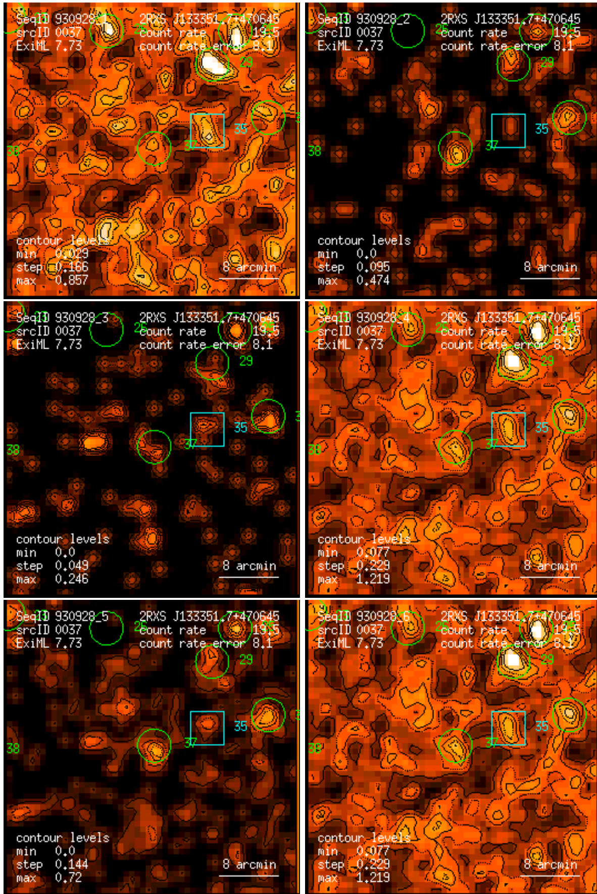
Figure 37: RASS 930928: detection 0037: band rate images, Gaussian filter: (1) PSPC channels 11 – 41, (2) 52 – 90, (3) 91 – 201, (4) 11 – 235, (5) 52 – 201, (6) 11 – 201. Broad band rates in counts/ks. Band rate contour levels in counts/ks/arcmin 2 .
