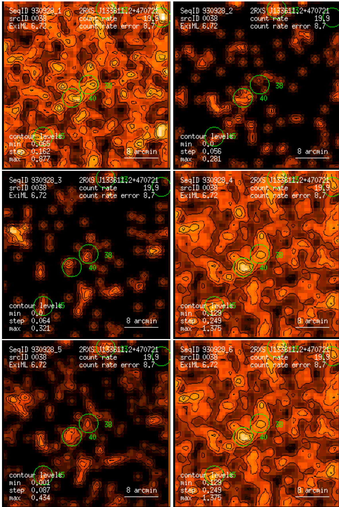
Figure 38: RASS 930928: detection 0038: band rate images, Gaussian filter: (1) PSPC channels 11 – 41, (2) 52 – 90, (3) 91 – 201, (4) 11 – 235, (5) 52 – 201, (6) 11 – 201. Broad band rates in counts/ks. Band rate contour levels in counts/ks/arcmin 2 .
