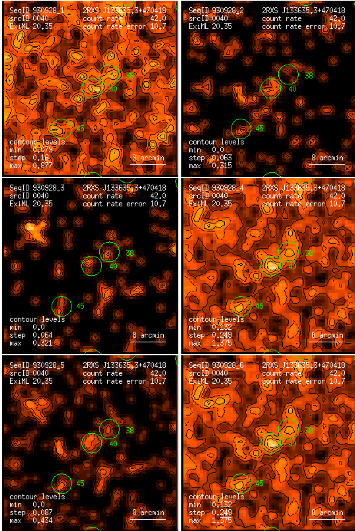
Figure 40: RASS 930928: detection 0040: band rate images, Gaussian filter: (1) PSPC channels 11 – 41, (2) 52 – 90, (3) 91 – 201, (4) 11 – 235, (5) 52 – 201, (6) 11 – 201. Broad band rates in counts/ks. Band rate contour levels in counts/ks/arcmin 2 .
