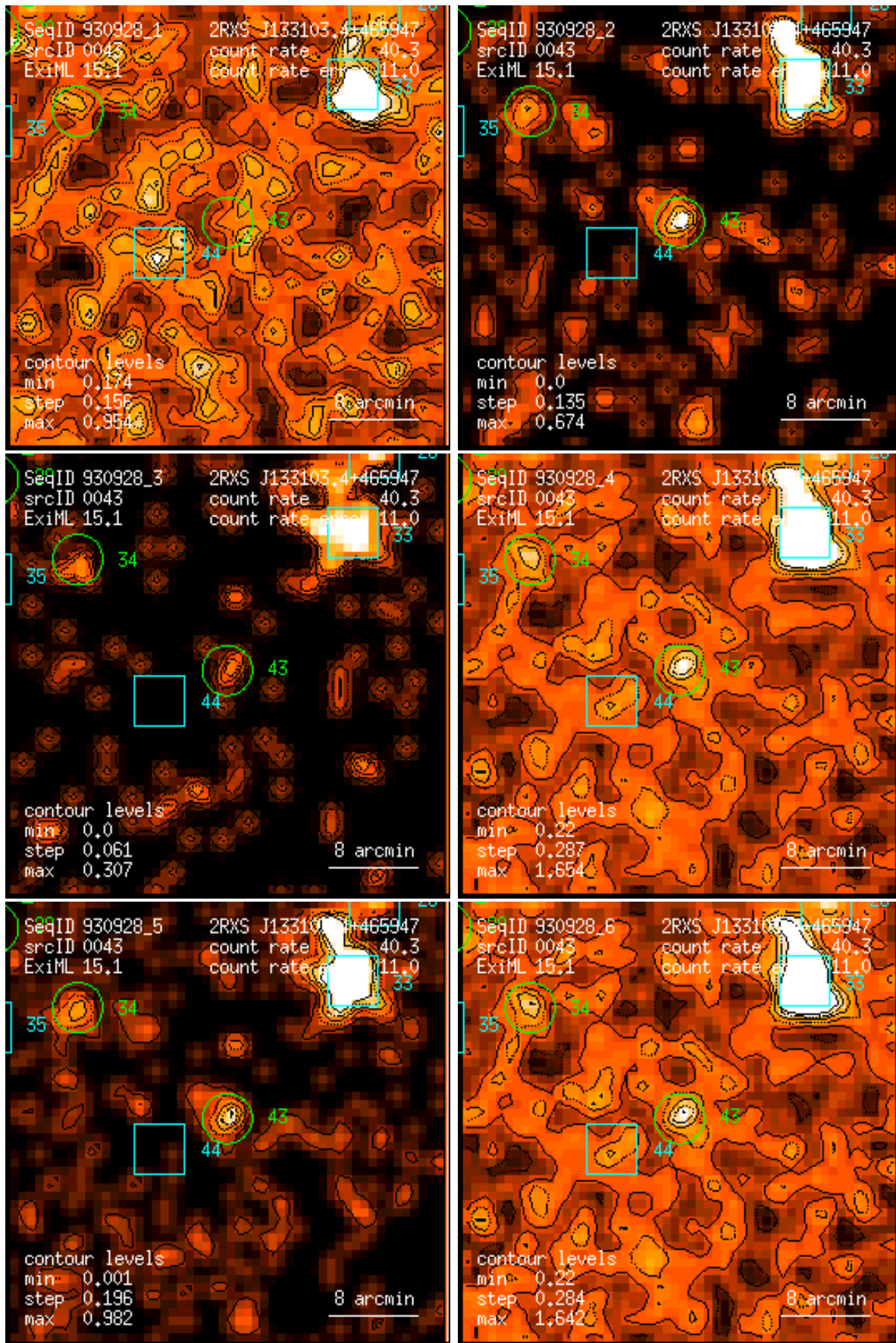
Figure 43: RASS 930928: detection 0043: band rate images, Gaussian filter: (1) PSPC channels 11 – 41, (2) 52 – 90, (3) 91 – 201, (4) 11 – 235, (5) 52 – 201, (6) 11 – 201. Broad band rates in counts/ks. Band rate contour levels in counts/ks/arcmin 2 .
