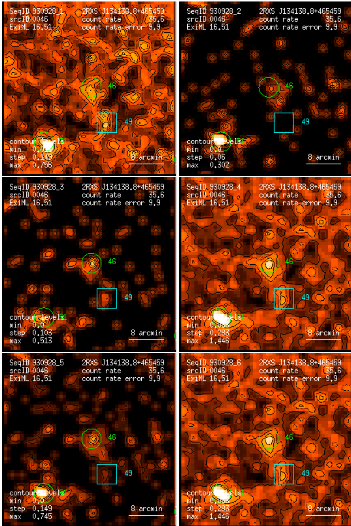
Figure 46: RASS 930928: detection 0046: band rate images, Gaussian filter: (1) PSPC channels 11 – 41, (2) 52 – 90, (3) 91 – 201, (4) 11 – 235, (5) 52 – 201, (6) 11 – 201. Broad band rates in counts/ks. Band rate contour levels in counts/ks/arcmin 2 .
