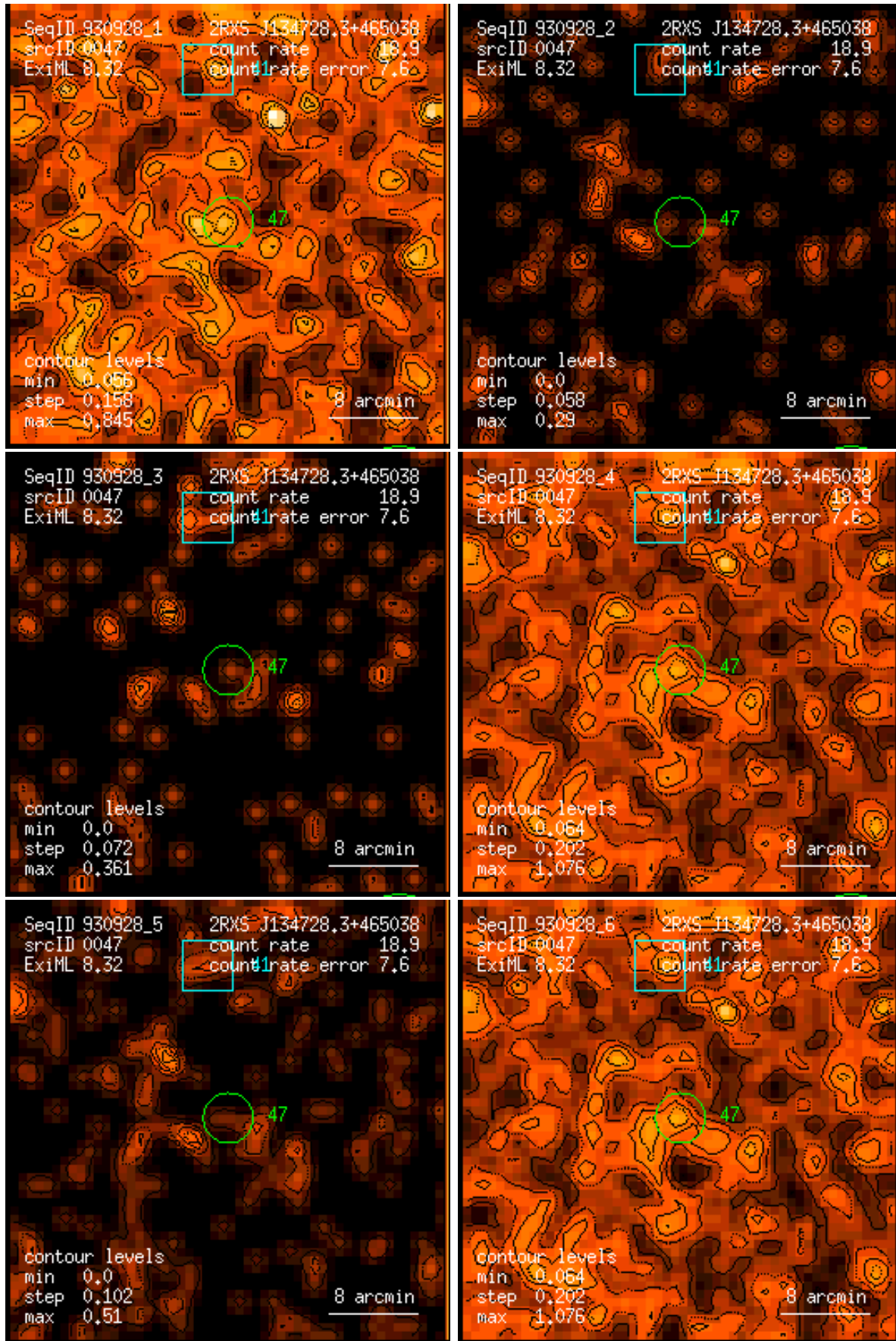
Figure 47: RASS 930928: detection 0047: band rate images, Gaussian filter: (1) PSPC channels 11 – 41, (2) 52 – 90, (3) 91 – 201, (4) 11 – 235, (5) 52 – 201, (6) 11 – 201. Broad band rates in counts/ks. Band rate contour levels in counts/ks/arcmin 2 .
