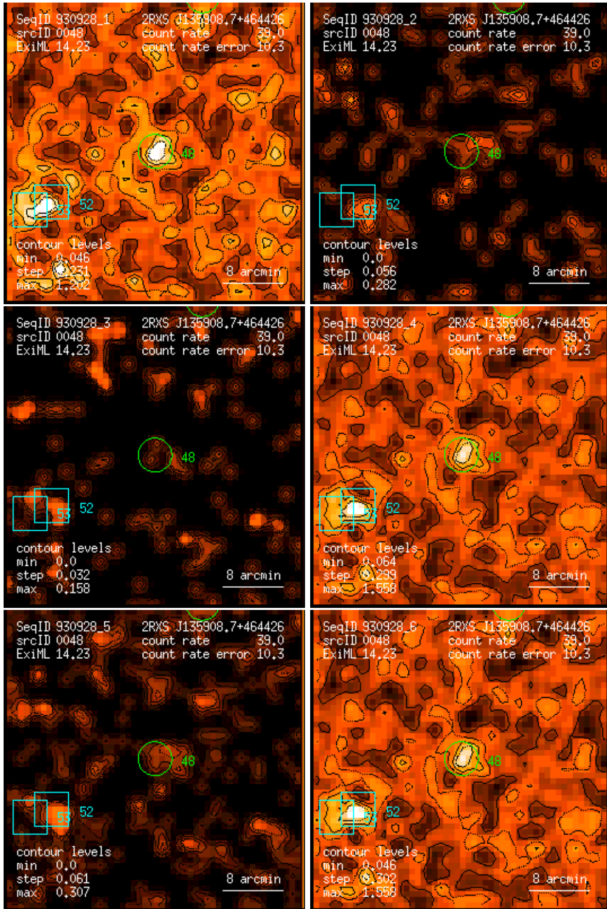
Figure 48: RASS 930928: detection 0048: band rate images, Gaussian filter: (1) PSPC channels 11 – 41, (2) 52 – 90, (3) 91 – 201, (4) 11 – 235, (5) 52 – 201, (6) 11 – 201. Broad band rates in counts/ks. Band rate contour levels in counts/ks/arcmin 2 .
