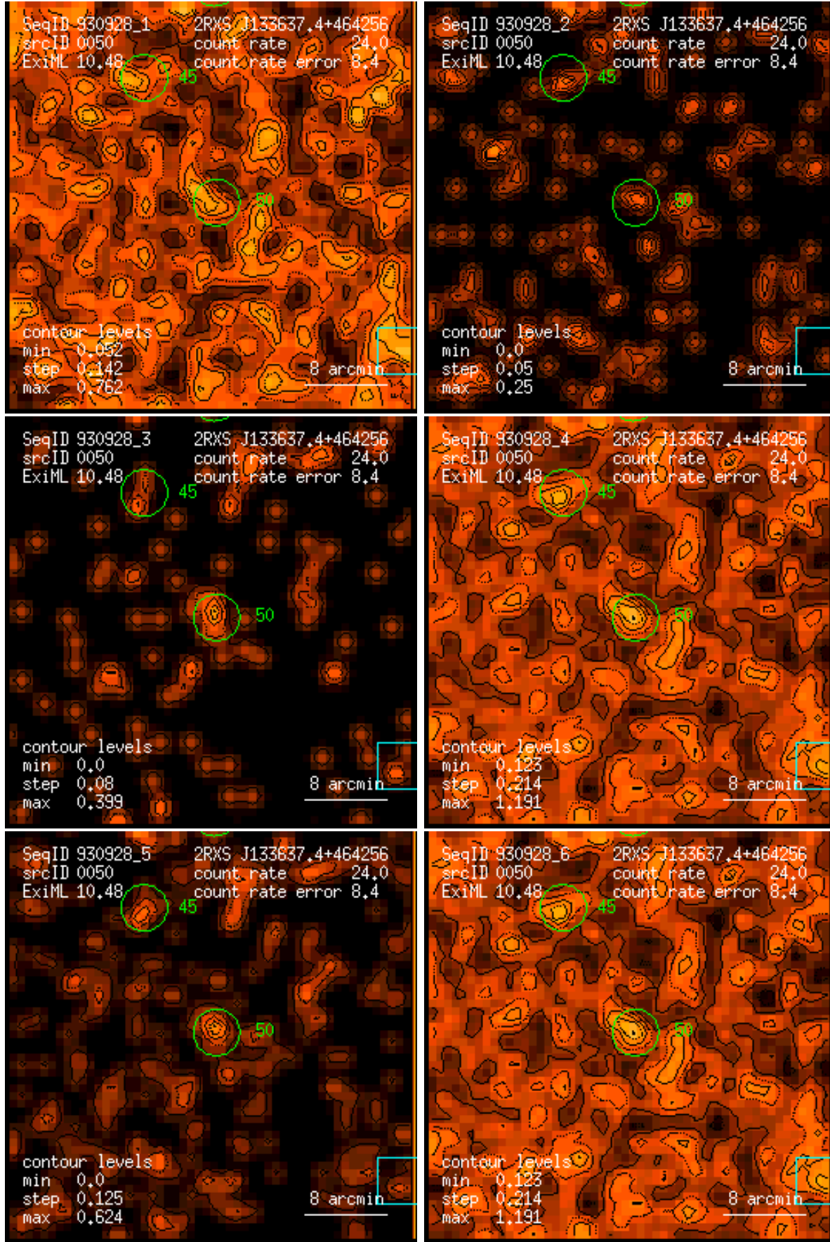
Figure 50: RASS 930928: detection 0050: band rate images, Gaussian filter: (1) PSPC channels 11 – 41, (2) 52 – 90, (3) 91 – 201, (4) 11 – 235, (5) 52 – 201, (6) 11 – 201. Broad band rates in counts/ks. Band rate contour levels in counts/ks/arcmin 2 .
