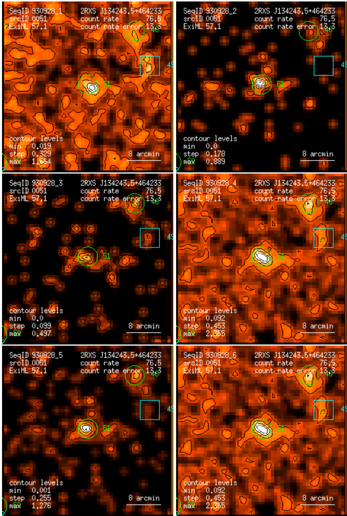
Figure 51: RASS 930928: detection 0051: band rate images, Gaussian filter: (1) PSPC channels 11 – 41, (2) 52 – 90, (3) 91 – 201, (4) 11 – 235, (5) 52 – 201, (6) 11 – 201. Broad band rates in counts/ks. Band rate contour levels in counts/ks/arcmin 2 .
