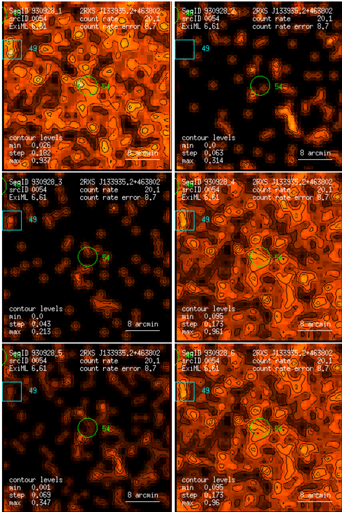
Figure 54: RASS 930928: detection 0054: band rate images, Gaussian filter: (1) PSPC channels 11 – 41, (2) 52 – 90, (3) 91 – 201, (4) 11 – 235, (5) 52 – 201, (6) 11 – 201. Broad band rates in counts/ks. Band rate contour levels in counts/ks/arcmin 2 .
