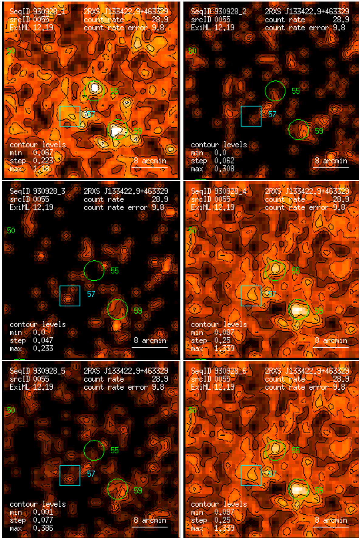
Figure 55: RASS 930928: detection 0055: band rate images, Gaussian filter: (1) PSPC channels 11 – 41, (2) 52 – 90, (3) 91 – 201, (4) 11 – 235, (5) 52 – 201, (6) 11 – 201. Broad band rates in counts/ks. Band rate contour levels in counts/ks/arcmin 2 .
