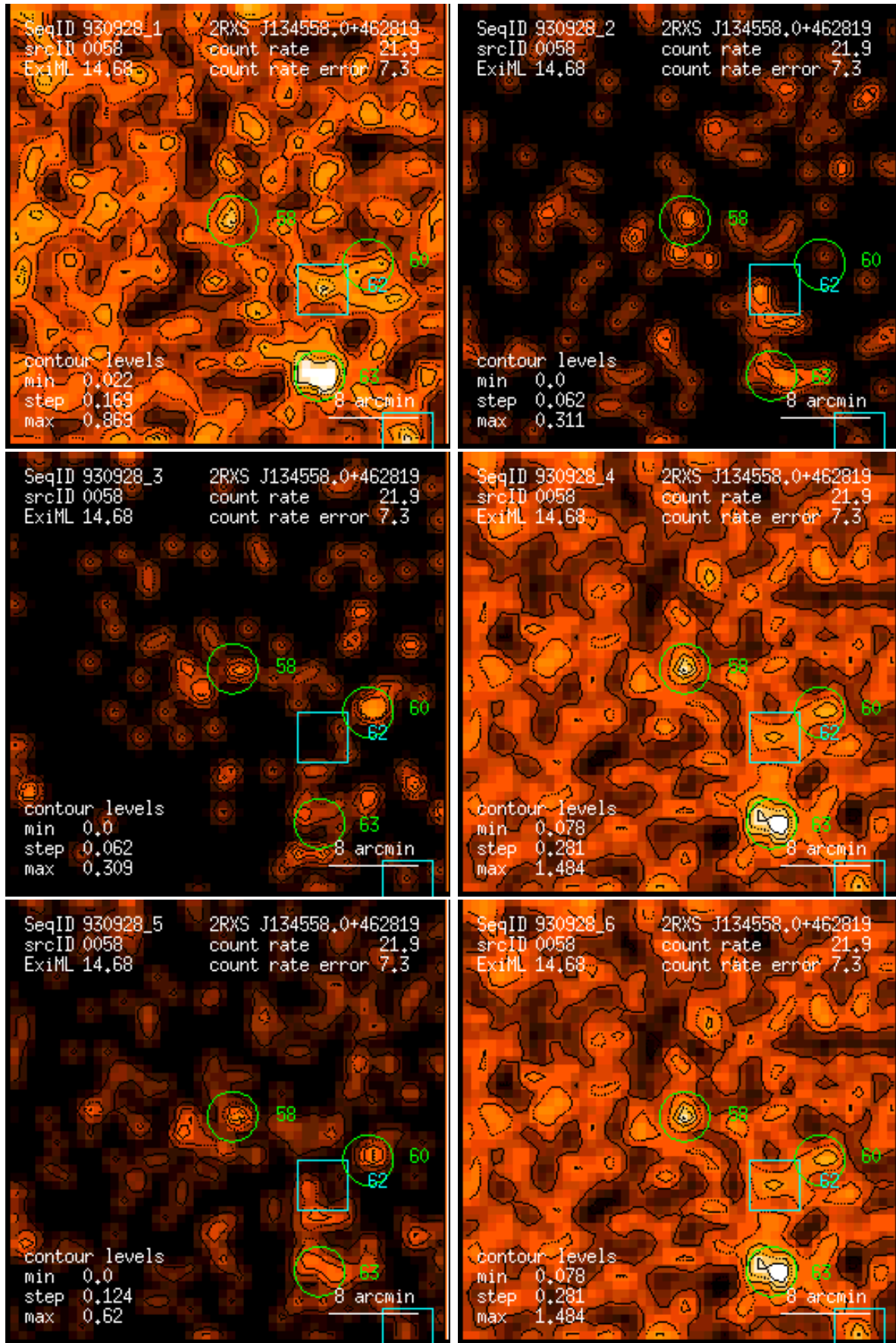
Figure 58: RASS 930928: detection 0058: band rate images, Gaussian filter: (1) PSPC channels 11 – 41, (2) 52 – 90, (3) 91 – 201, (4) 11 – 235, (5) 52 – 201, (6) 11 – 201. Broad band rates in counts/ks. Band rate contour levels in counts/ks/arcmin 2 .
