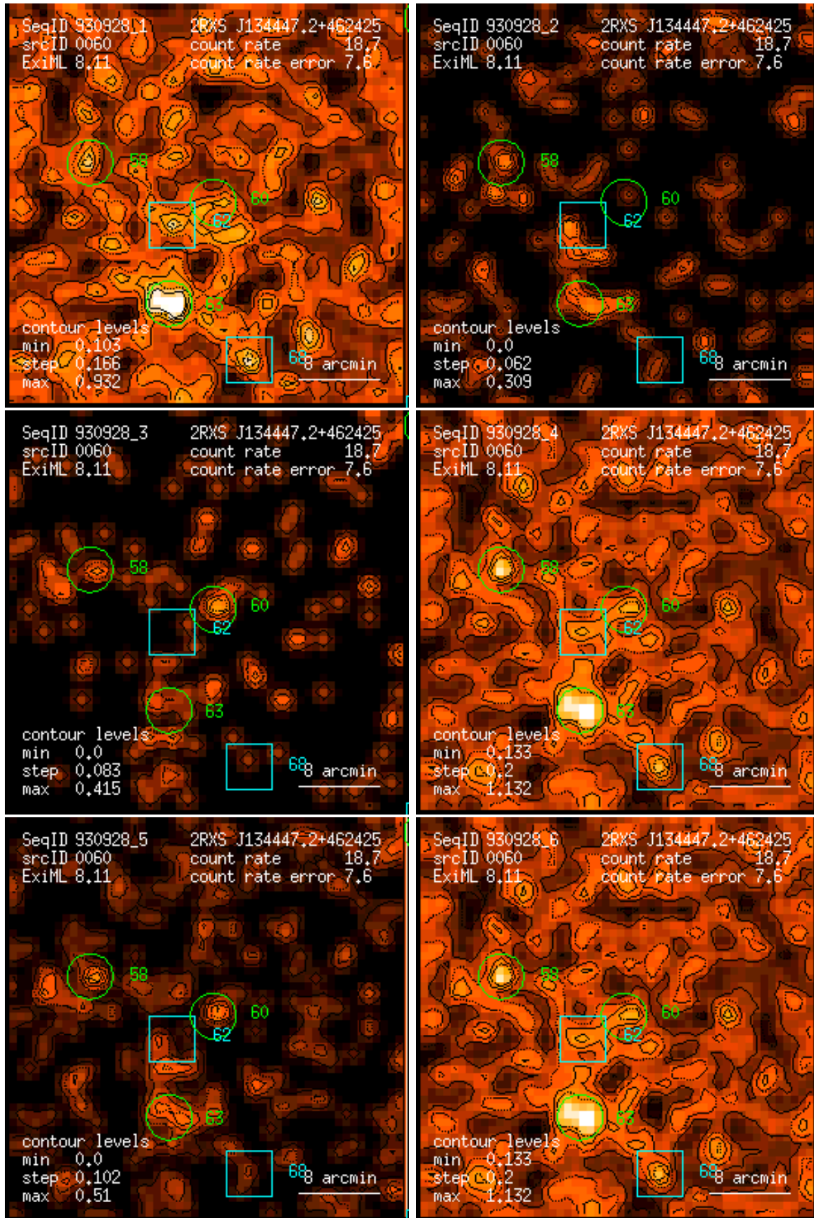
Figure 60: RASS 930928: detection 0060: band rate images, Gaussian filter: (1) PSPC channels 11 – 41, (2) 52 – 90, (3) 91 – 201, (4) 11 – 235, (5) 52 – 201, (6) 11 – 201. Broad band rates in counts/ks. Band rate contour levels in counts/ks/arcmin 2 .
