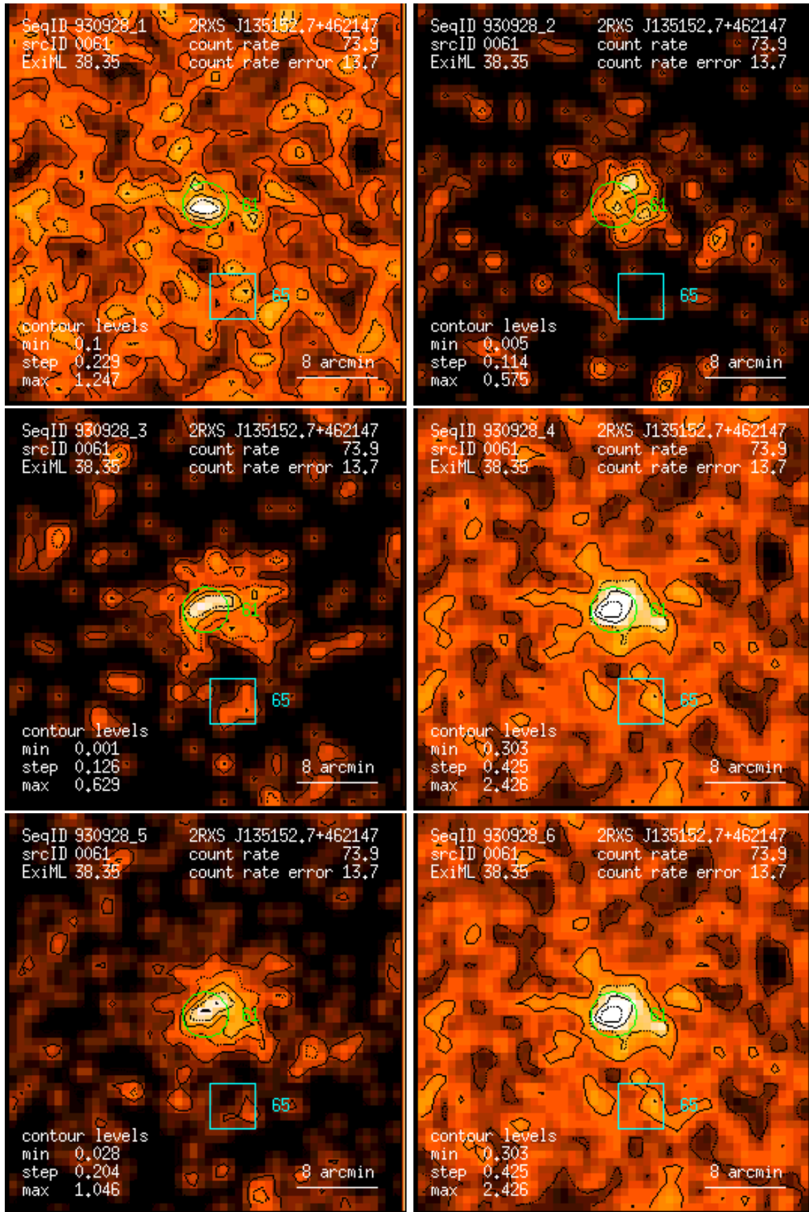
Figure 61: RASS 930928: detection 0061: band rate images, Gaussian filter: (1) PSPC channels 11 – 41, (2) 52 – 90, (3) 91 – 201, (4) 11 – 235, (5) 52 – 201, (6) 11 – 201. Broad band rates in counts/ks. Band rate contour levels in counts/ks/arcmin 2 .
