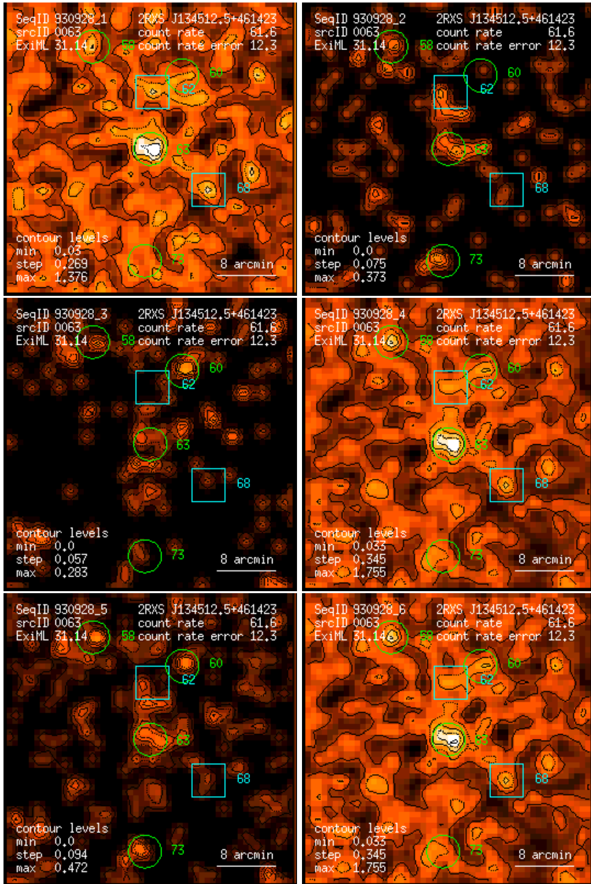
Figure 63: RASS 930928: detection 0063: band rate images, Gaussian filter: (1) PSPC channels 11 – 41, (2) 52 – 90, (3) 91 – 201, (4) 11 – 235, (5) 52 – 201, (6) 11 – 201. Broad band rates in counts/ks. Band rate contour levels in counts/ks/arcmin 2 .
