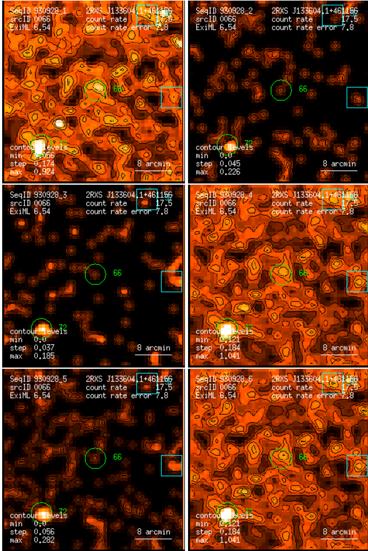
Figure 66: RASS 930928: detection 0066: band rate images, Gaussian filter: (1) PSPC channels 11 – 41, (2) 52 – 90, (3) 91 – 201, (4) 11 – 235, (5) 52 – 201, (6) 11 – 201. Broad band rates in counts/ks. Band rate contour levels in counts/ks/arcmin 2 .
