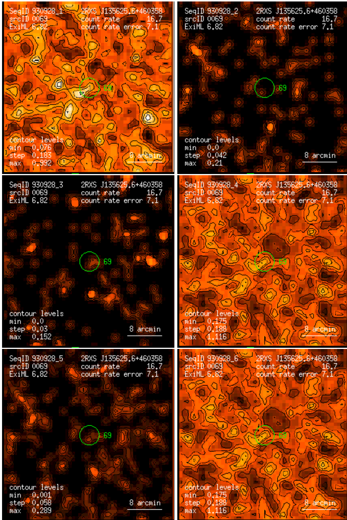
Figure 69: RASS 930928: detection 0069: band rate images, Gaussian filter: (1) PSPC channels 11 – 41, (2) 52 – 90, (3) 91 – 201, (4) 11 – 235, (5) 52 – 201, (6) 11 – 201. Broad band rates in counts/ks. Band rate contour levels in counts/ks/arcmin 2 .
