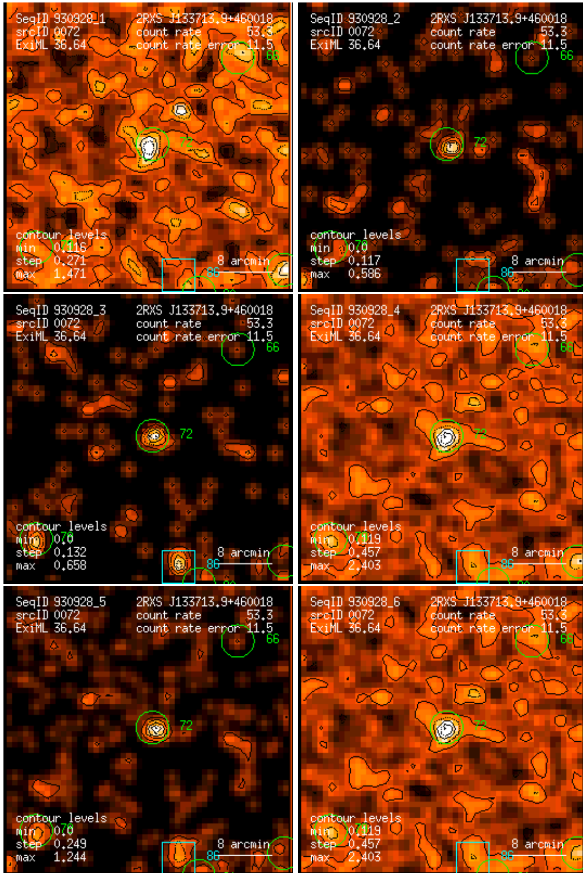
Figure 72: RASS 930928: detection 0072: band rate images, Gaussian filter: (1) PSPC channels 11 – 41, (2) 52 – 90, (3) 91 – 201, (4) 11 – 235, (5) 52 – 201, (6) 11 – 201. Broad band rates in counts/ks. Band rate contour levels in counts/ks/arcmin 2 .
