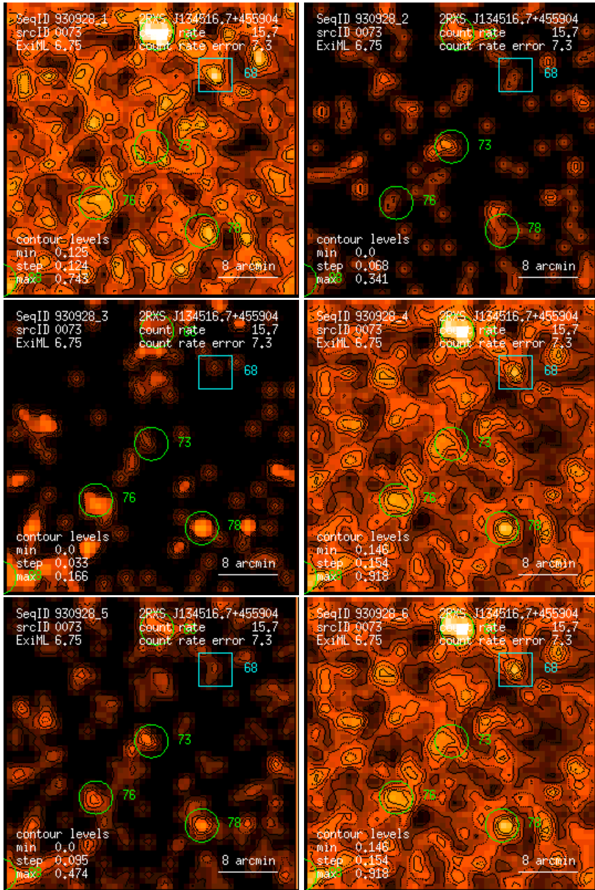
Figure 73: RASS 930928: detection 0073: band rate images, Gaussian filter: (1) PSPC channels 11 – 41, (2) 52 – 90, (3) 91 – 201, (4) 11 – 235, (5) 52 – 201, (6) 11 – 201. Broad band rates in counts/ks. Band rate contour levels in counts/ks/arcmin 2 .
