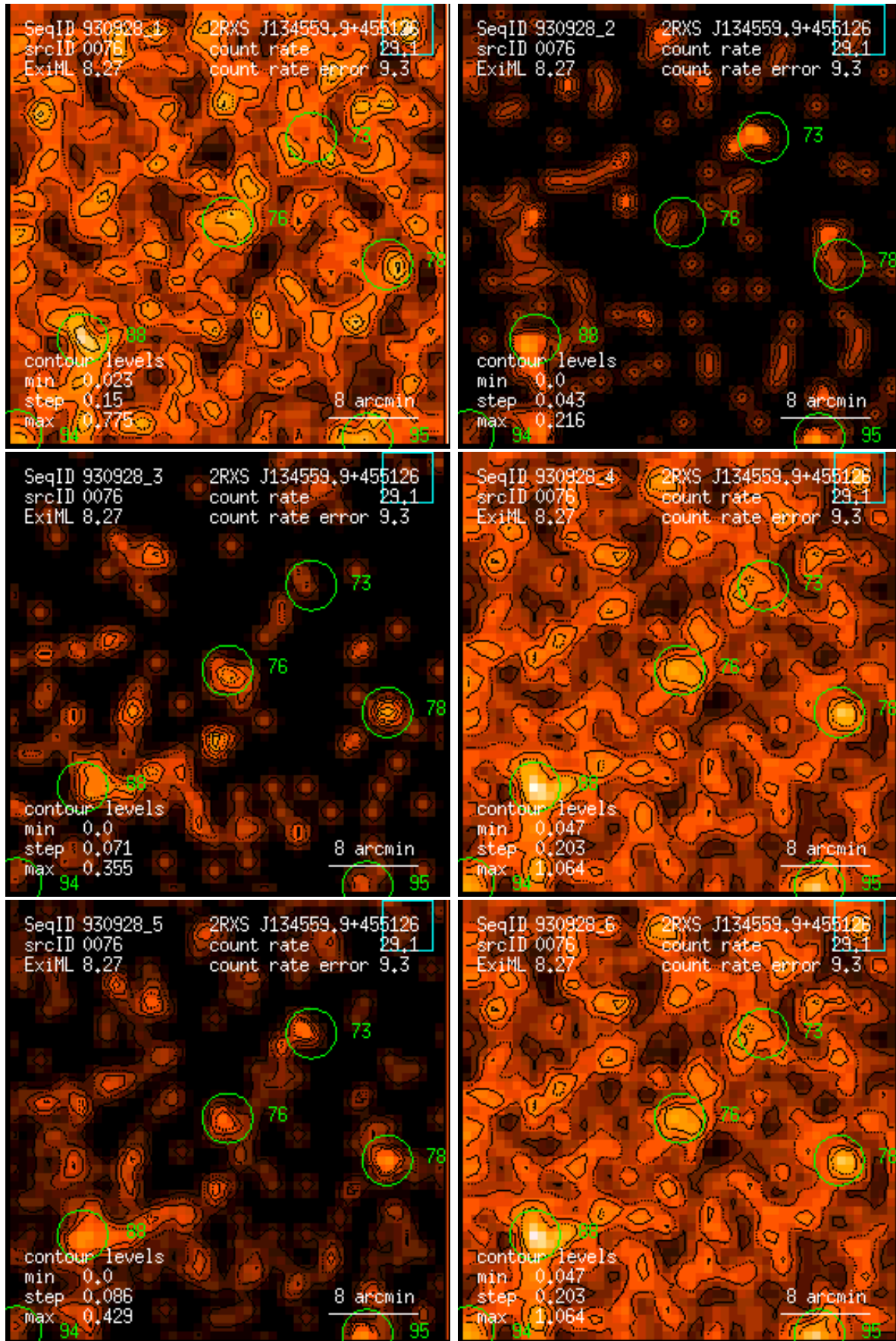
Figure 76: RASS 930928: detection 0076: band rate images, Gaussian filter: (1) PSPC channels 11 – 41, (2) 52 – 90, (3) 91 – 201, (4) 11 – 235, (5) 52 – 201, (6) 11 – 201. Broad band rates in counts/ks. Band rate contour levels in counts/ks/arcmin 2 .
