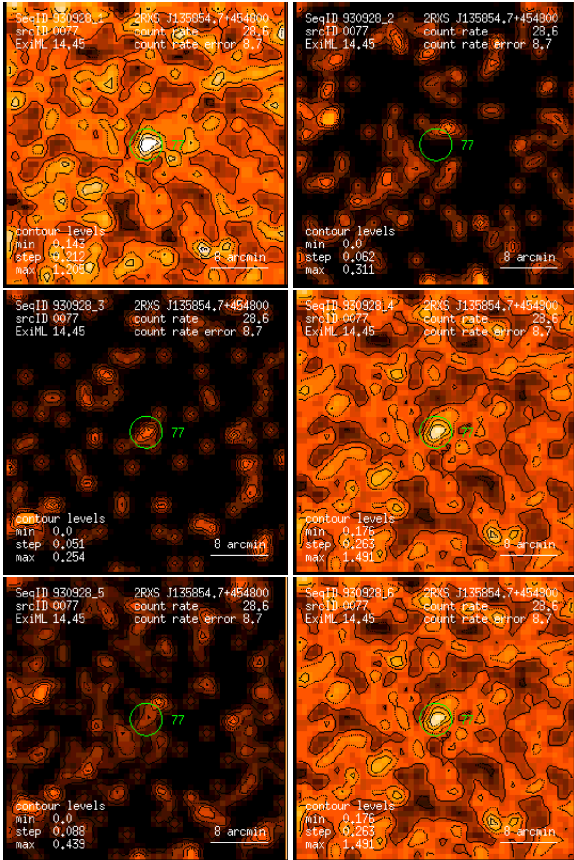
Figure 77: RASS 930928: detection 0077: band rate images, Gaussian filter: (1) PSPC channels 11 – 41, (2) 52 – 90, (3) 91 – 201, (4) 11 – 235, (5) 52 – 201, (6) 11 – 201. Broad band rates in counts/ks. Band rate contour levels in counts/ks/arcmin 2 .
