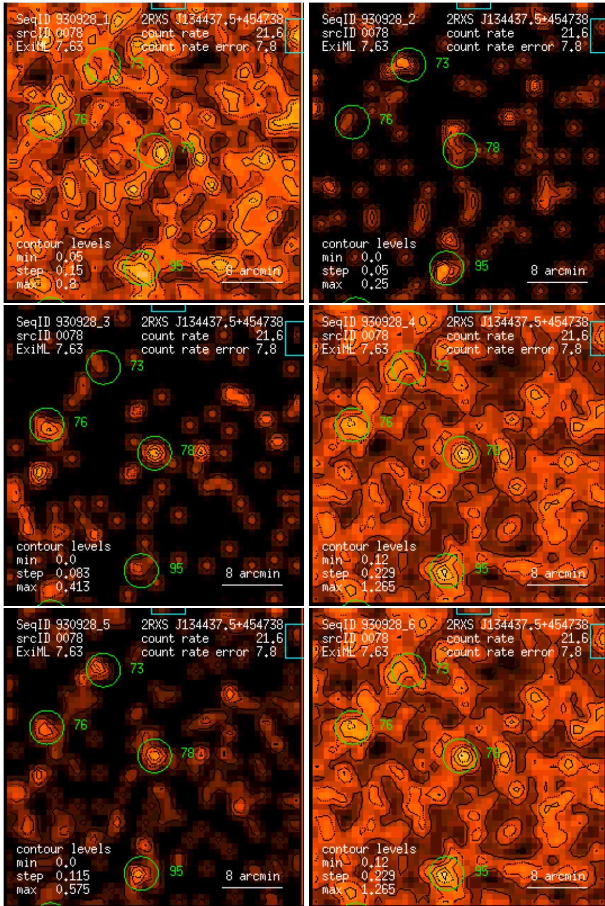
Figure 78: RASS 930928: detection 0078: band rate images, Gaussian filter: (1) PSPC channels 11 – 41, (2) 52 – 90, (3) 91 – 201, (4) 11 – 235, (5) 52 – 201, (6) 11 – 201. Broad band rates in counts/ks. Band rate contour levels in counts/ks/arcmin 2 .
