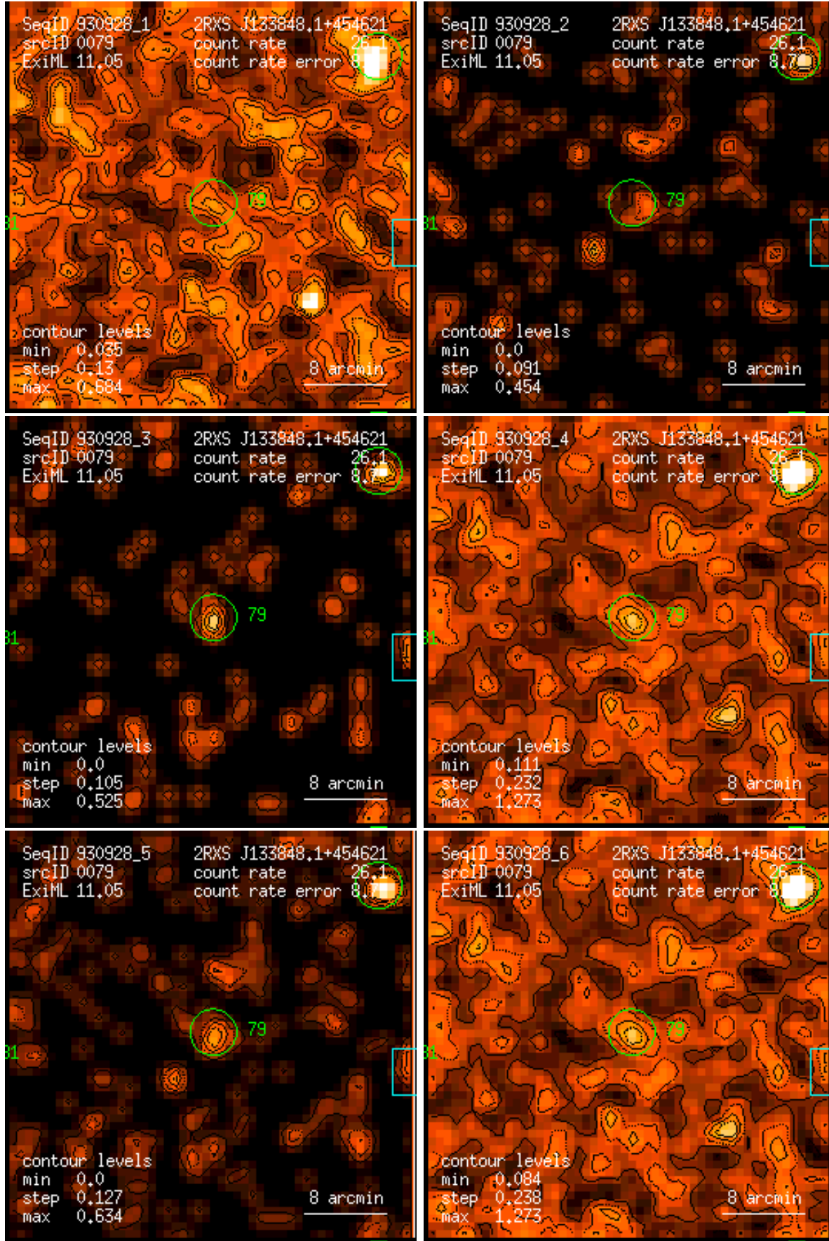
Figure 79: RASS 930928: detection 0079: band rate images, Gaussian filter: (1) PSPC channels 11 – 41, (2) 52 – 90, (3) 91 – 201, (4) 11 – 235, (5) 52 – 201, (6) 11 – 201. Broad band rates in counts/ks. Band rate contour levels in counts/ks/arcmin 2 .
